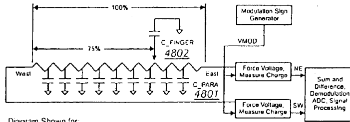
Diagram Shown for: "Measure X" On C_PARA is parasitic capacitance distributed across touch panel. "Measure XY" On C_FINGER is signal capacitance associated with a touch on the touch panel. "Measure Y" Off
