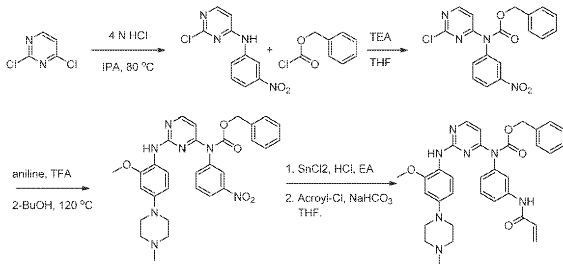
5 Scheme 3.
