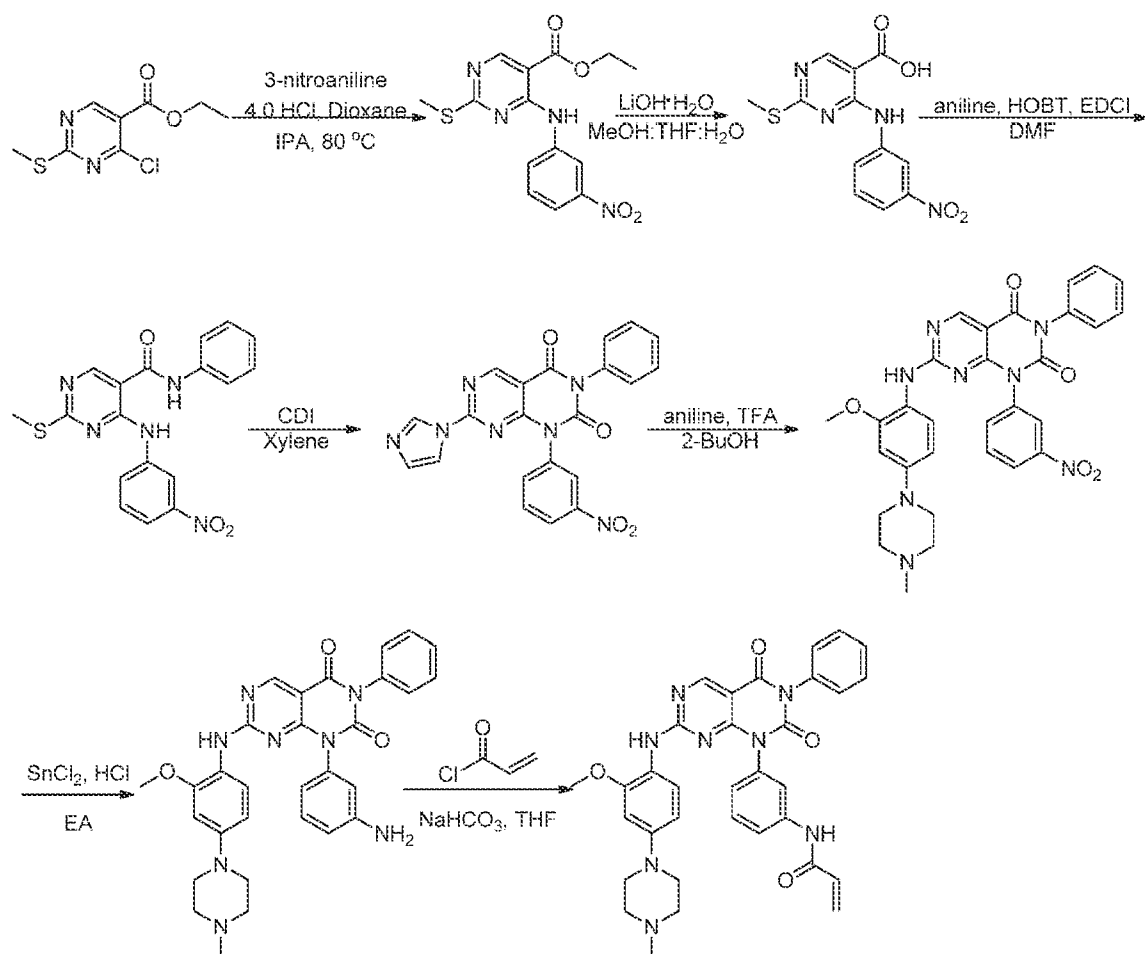
Scheme 5.
