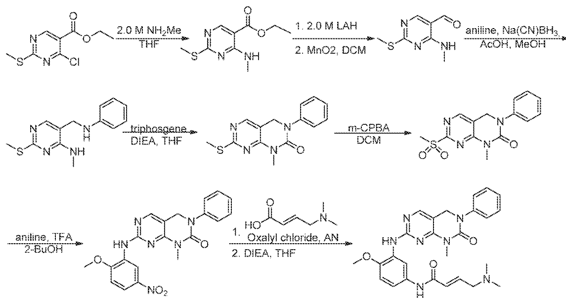
Scheme 6.
