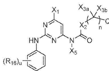
(VIa),
