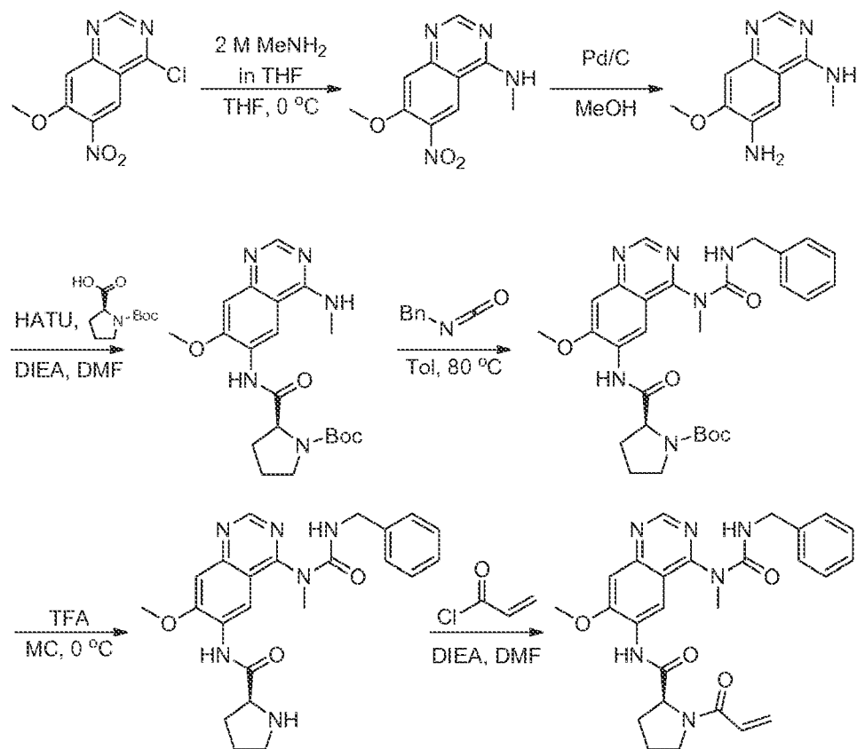
Scheme 4.
