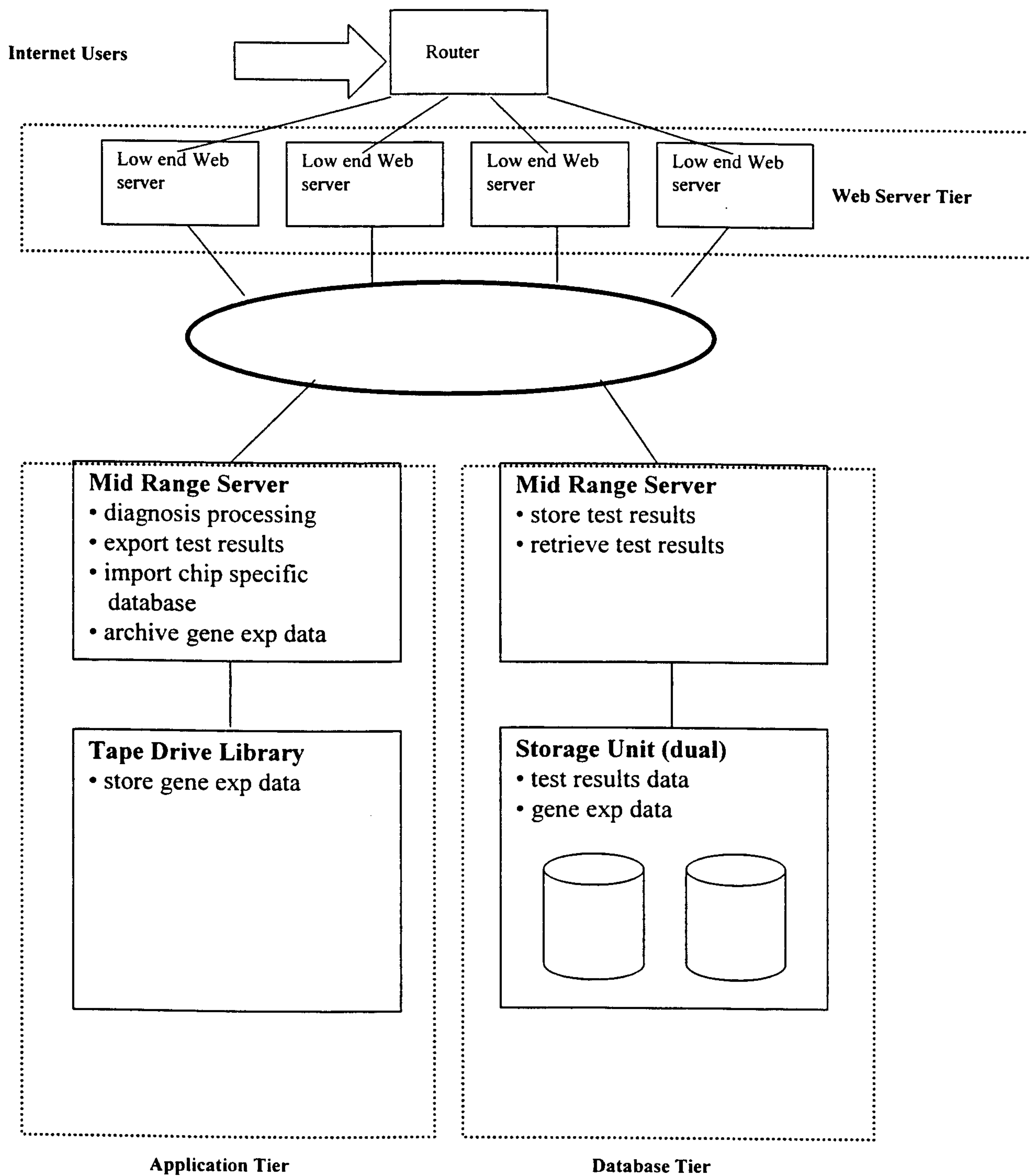
Figure 2: System Design
