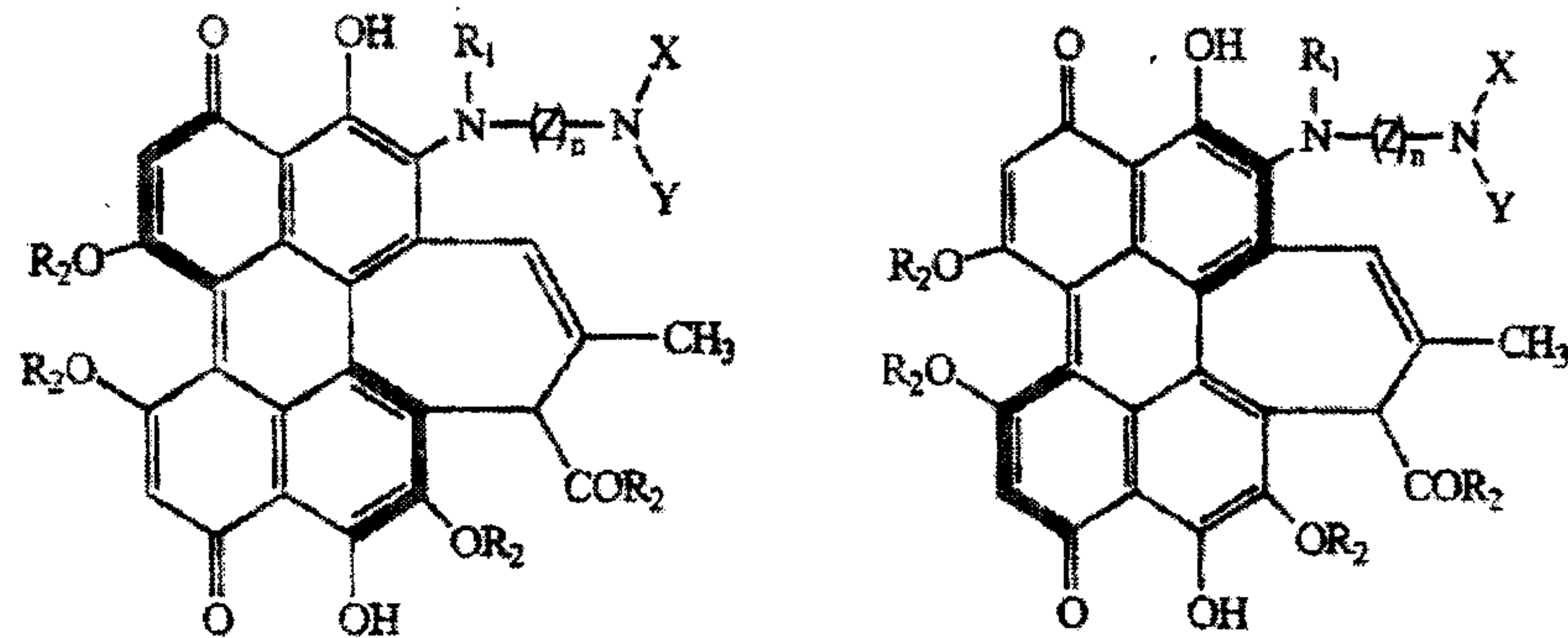
Atropisomers of (Ia)
