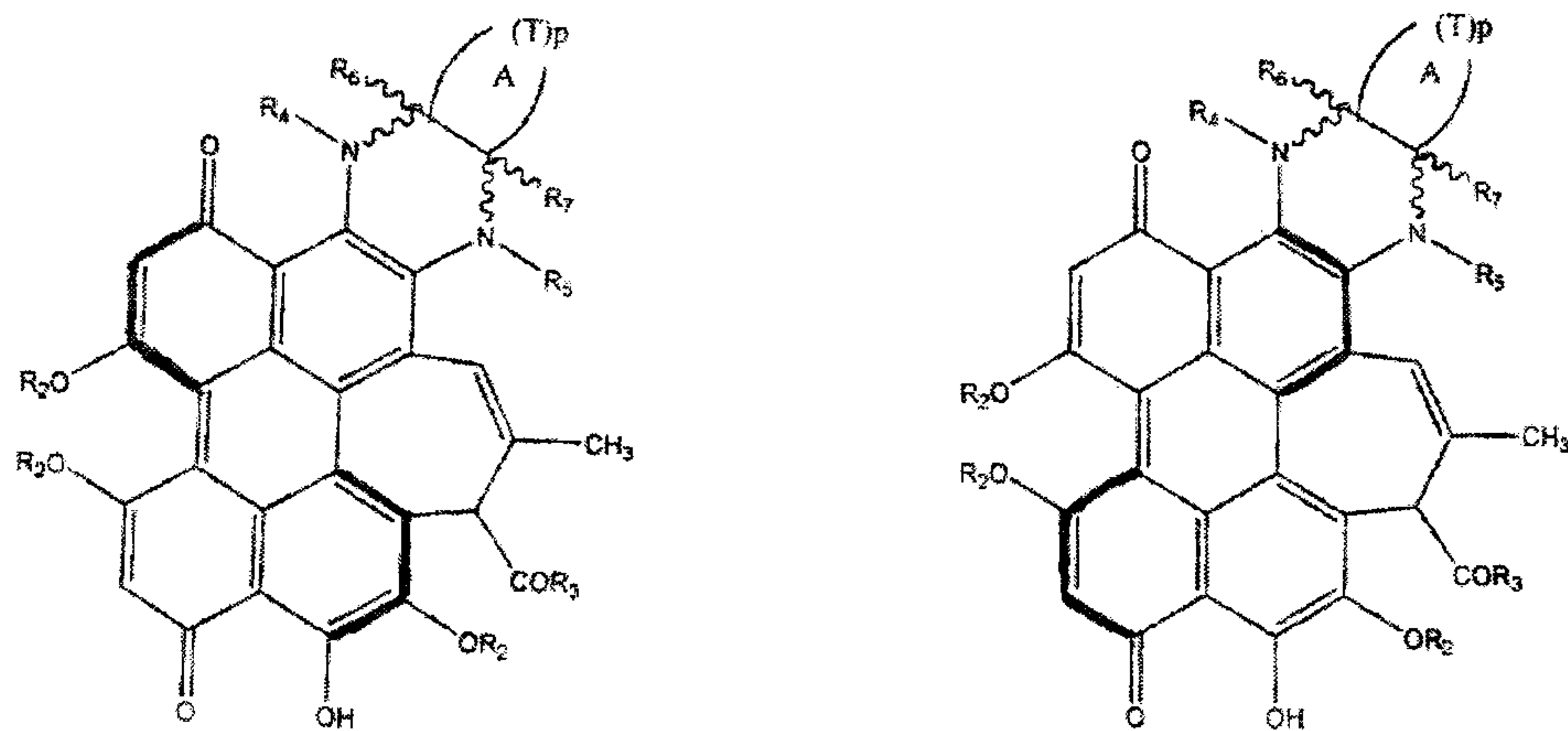
Atropisomers of (IIIa)
