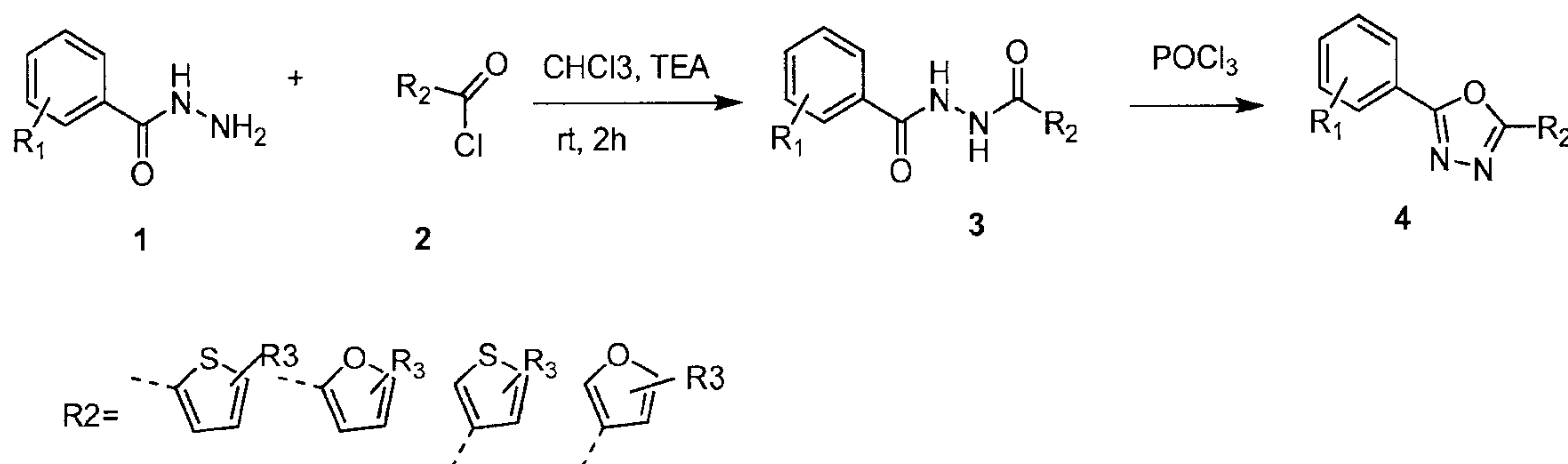
10 Scheme 3: Synthetic scheme to compounds of the Formula IIIa and IIIb
