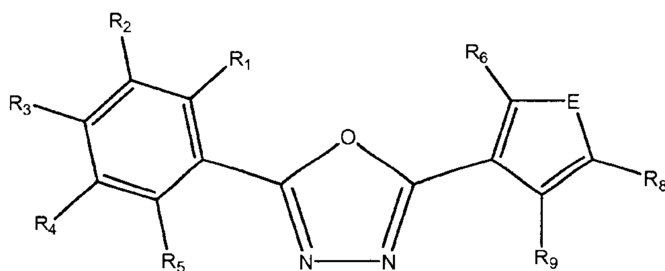
Formula IIIb
