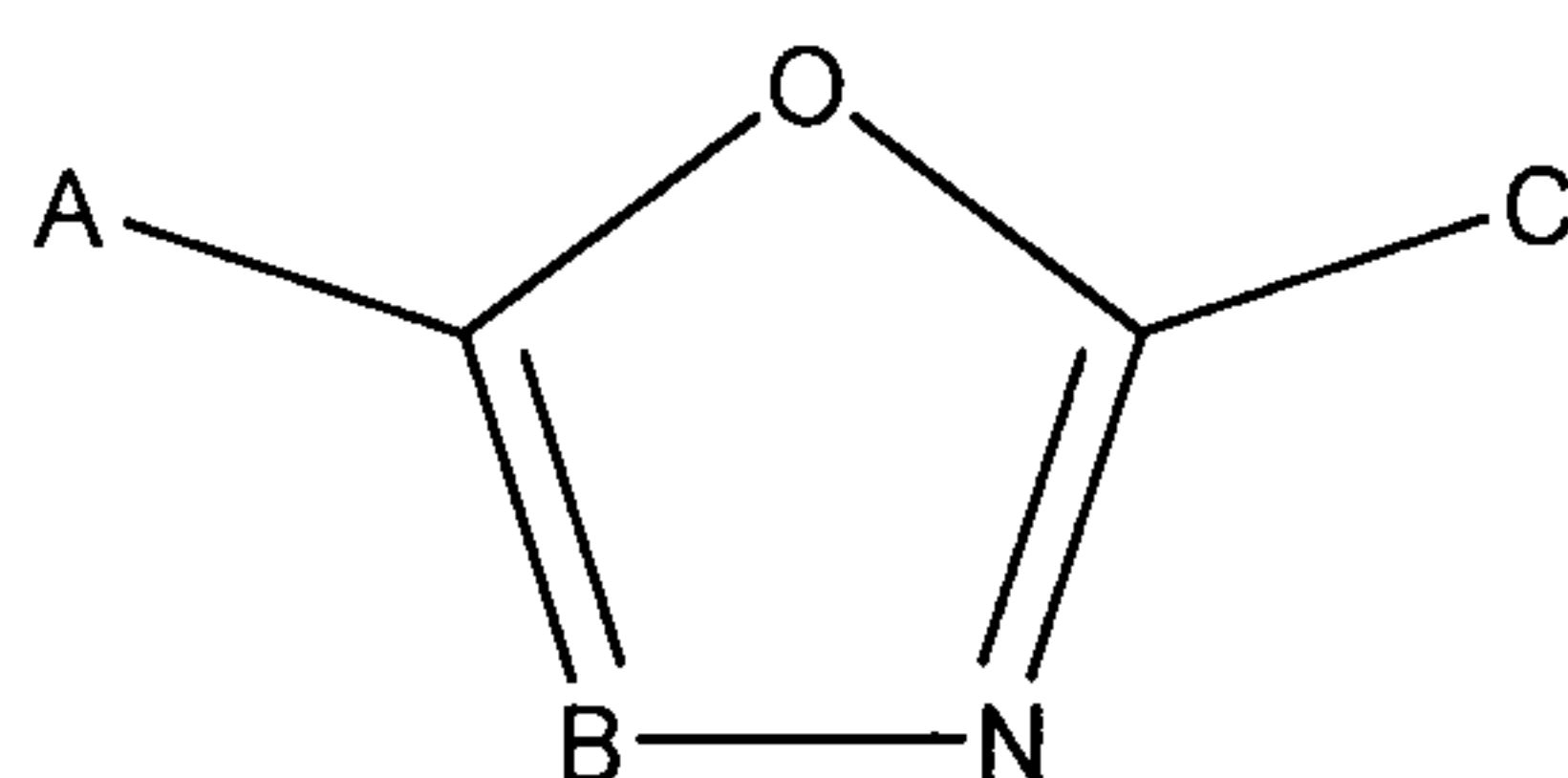
Formula I
