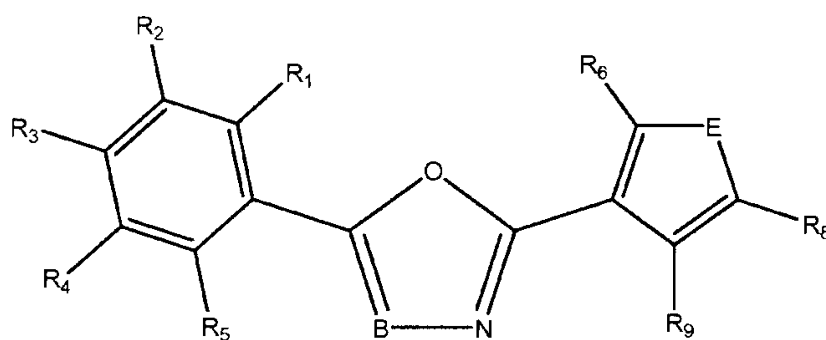
Formula Ib
