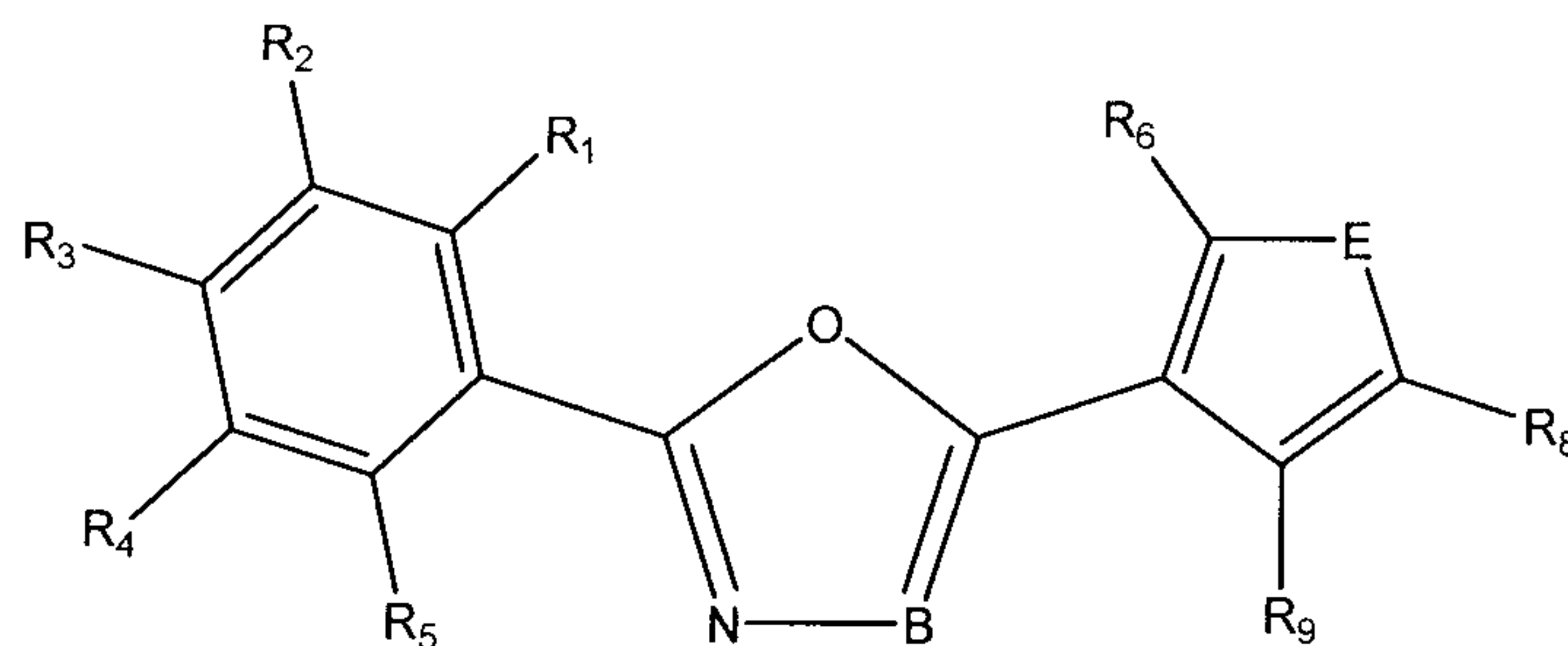
Formula IIb
