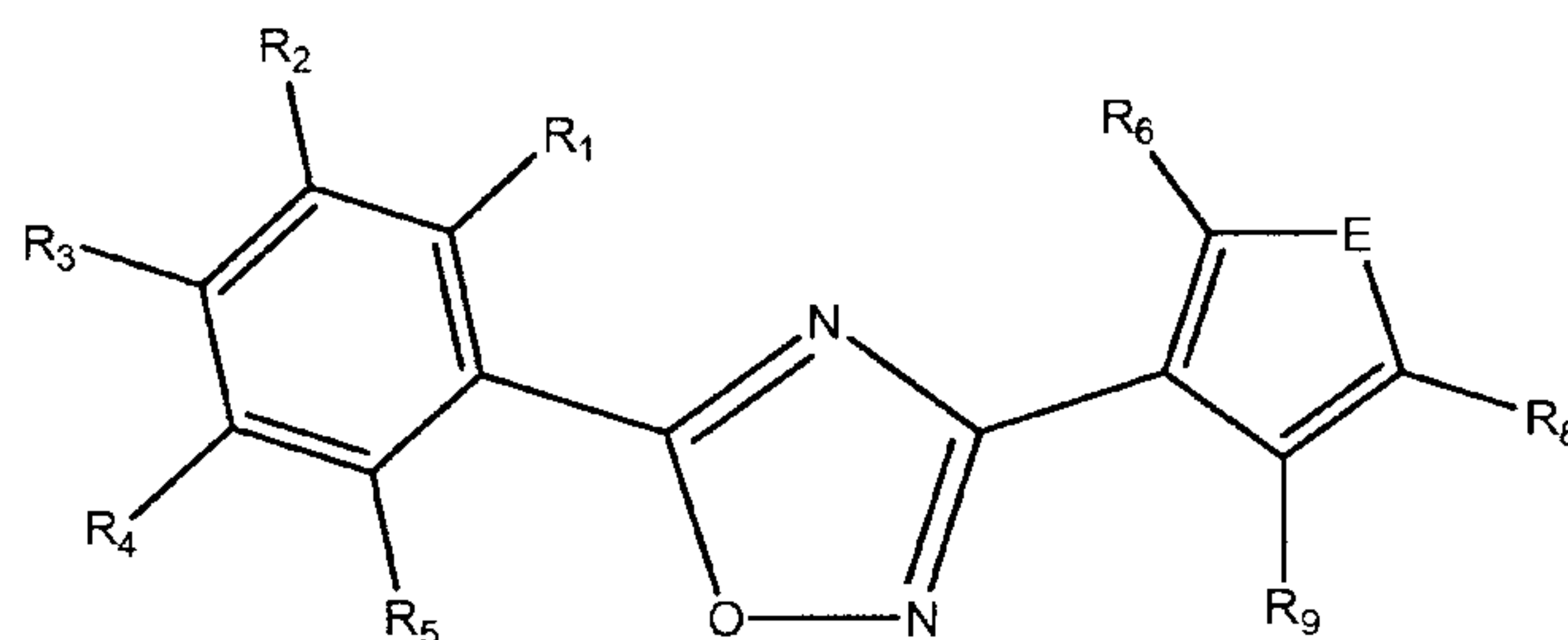
Formula Vb
