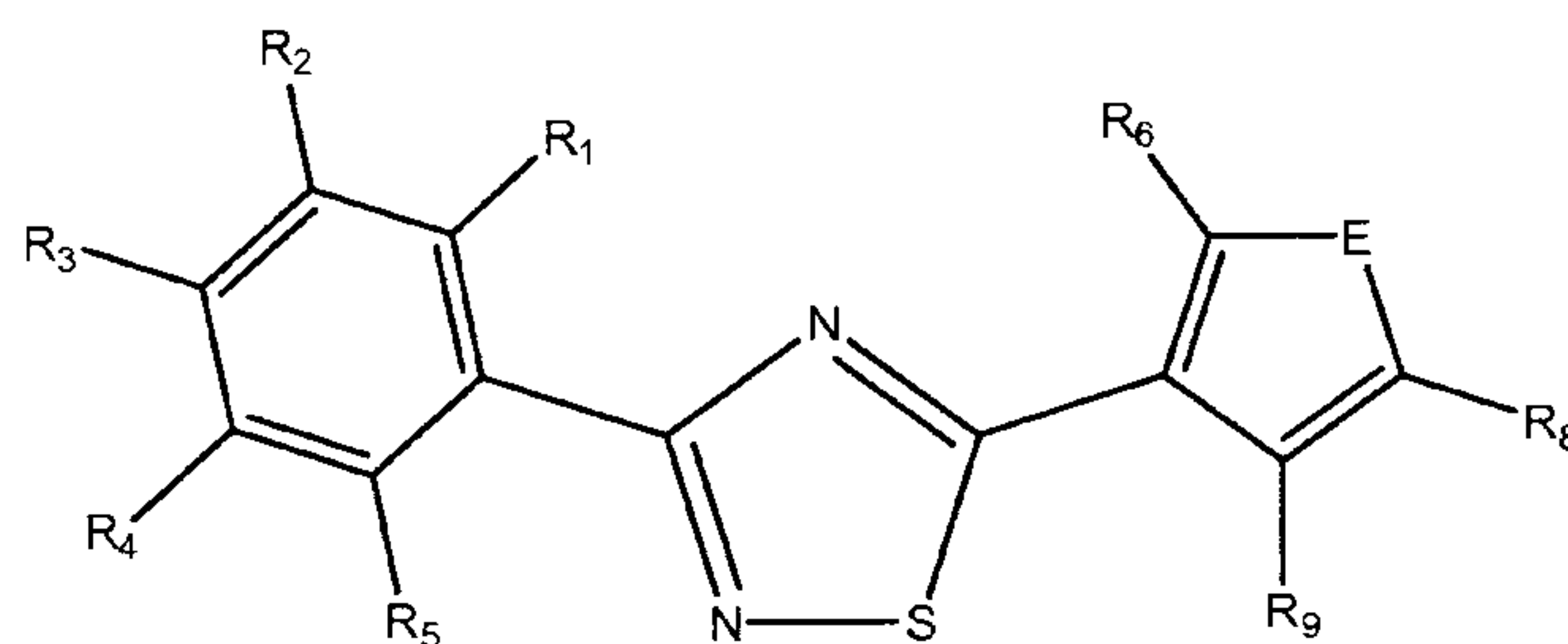
Formula VIb
