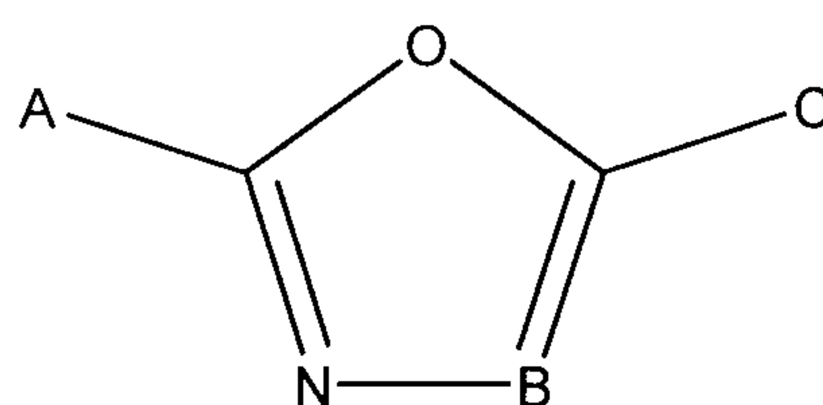
Formula II
