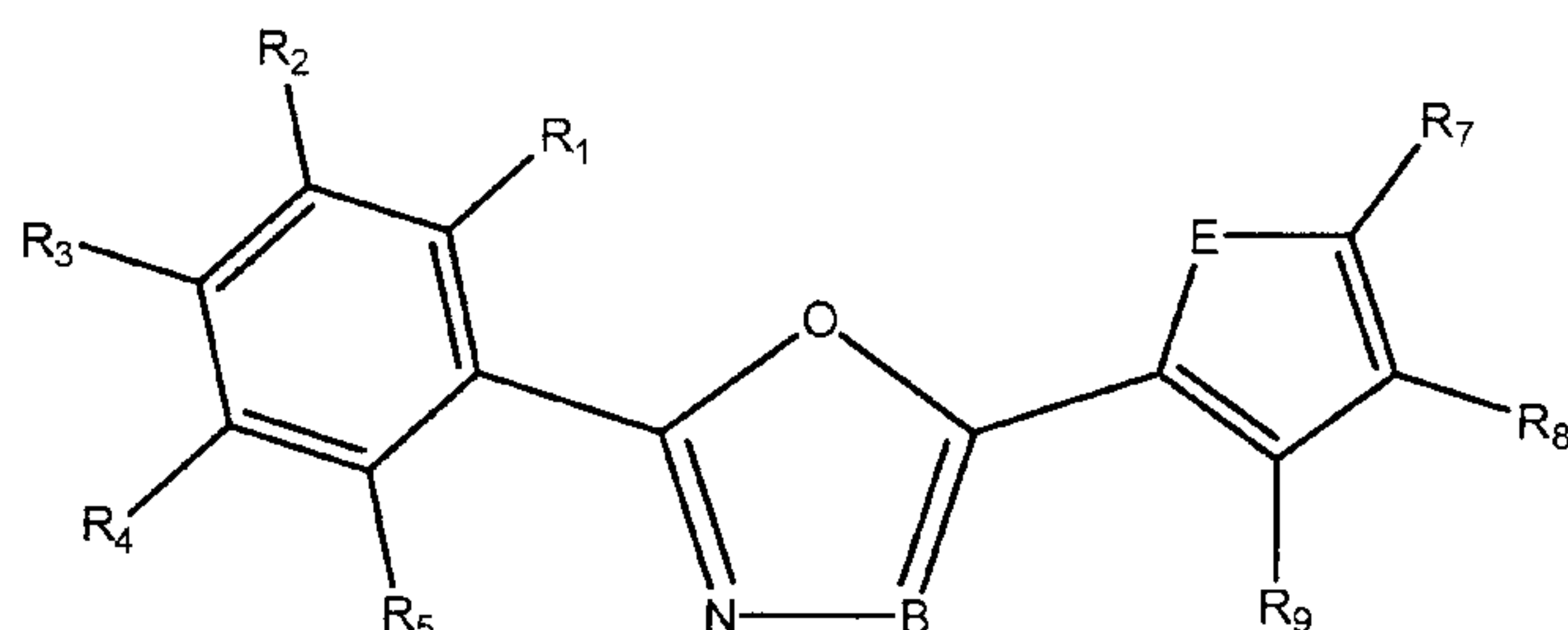
Formula IIa
