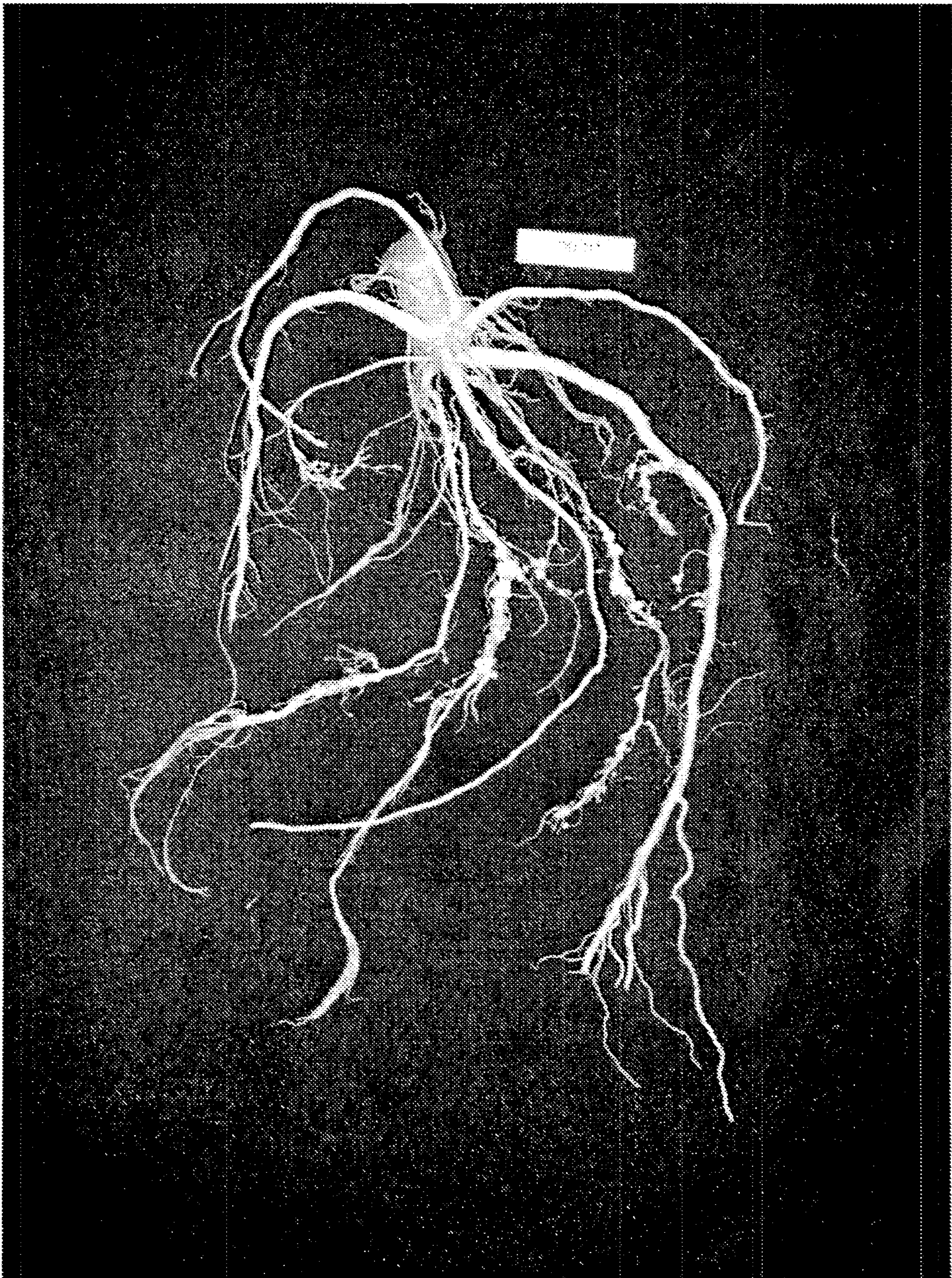
Figure 1: Roots from non-treated plants (Fall trial)
