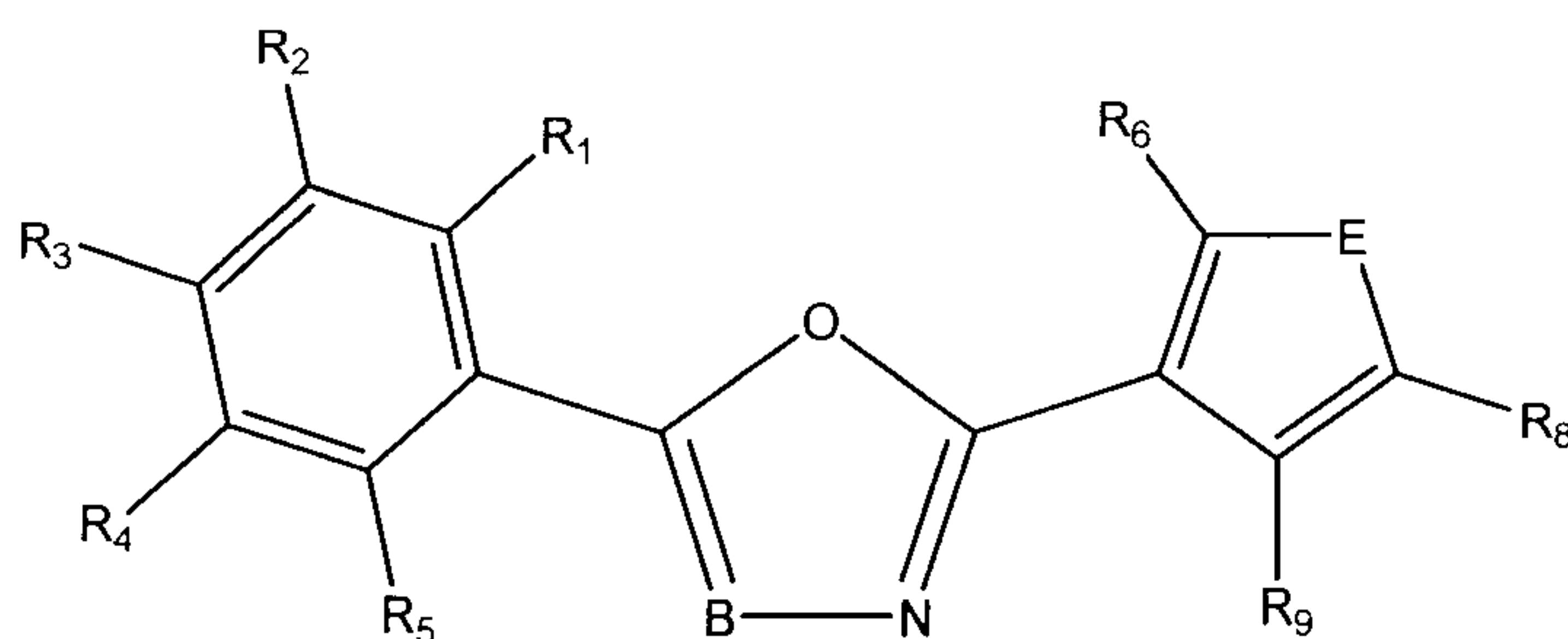
Formula Ib
