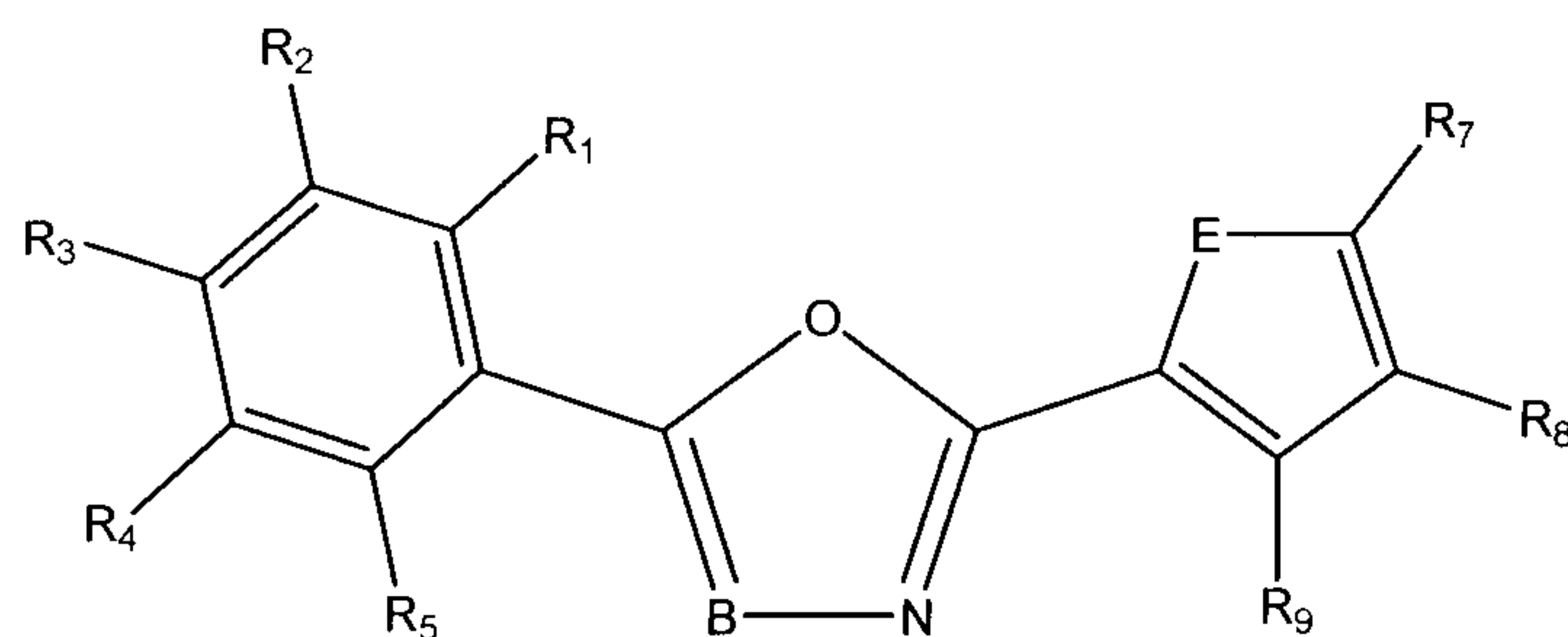
Formula Ia
