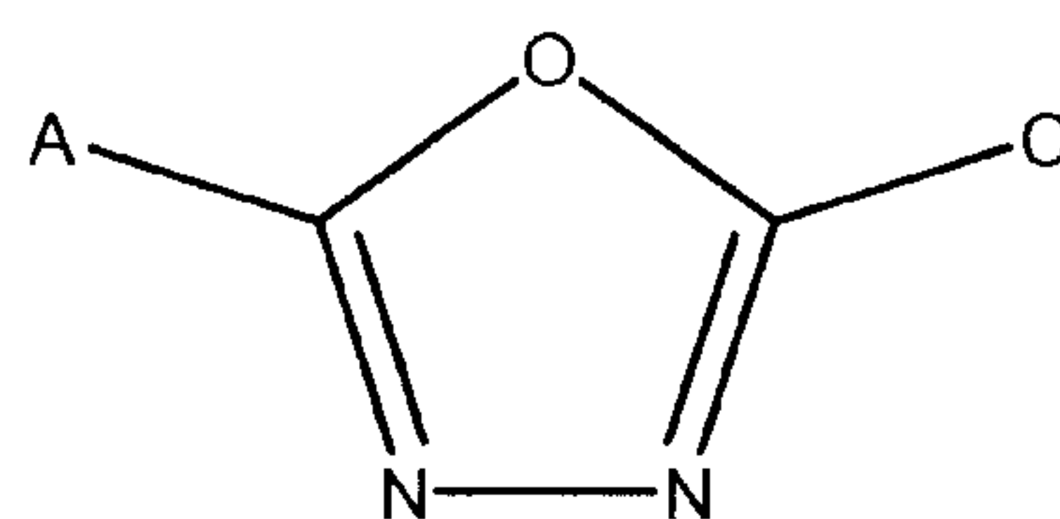
Formula III
