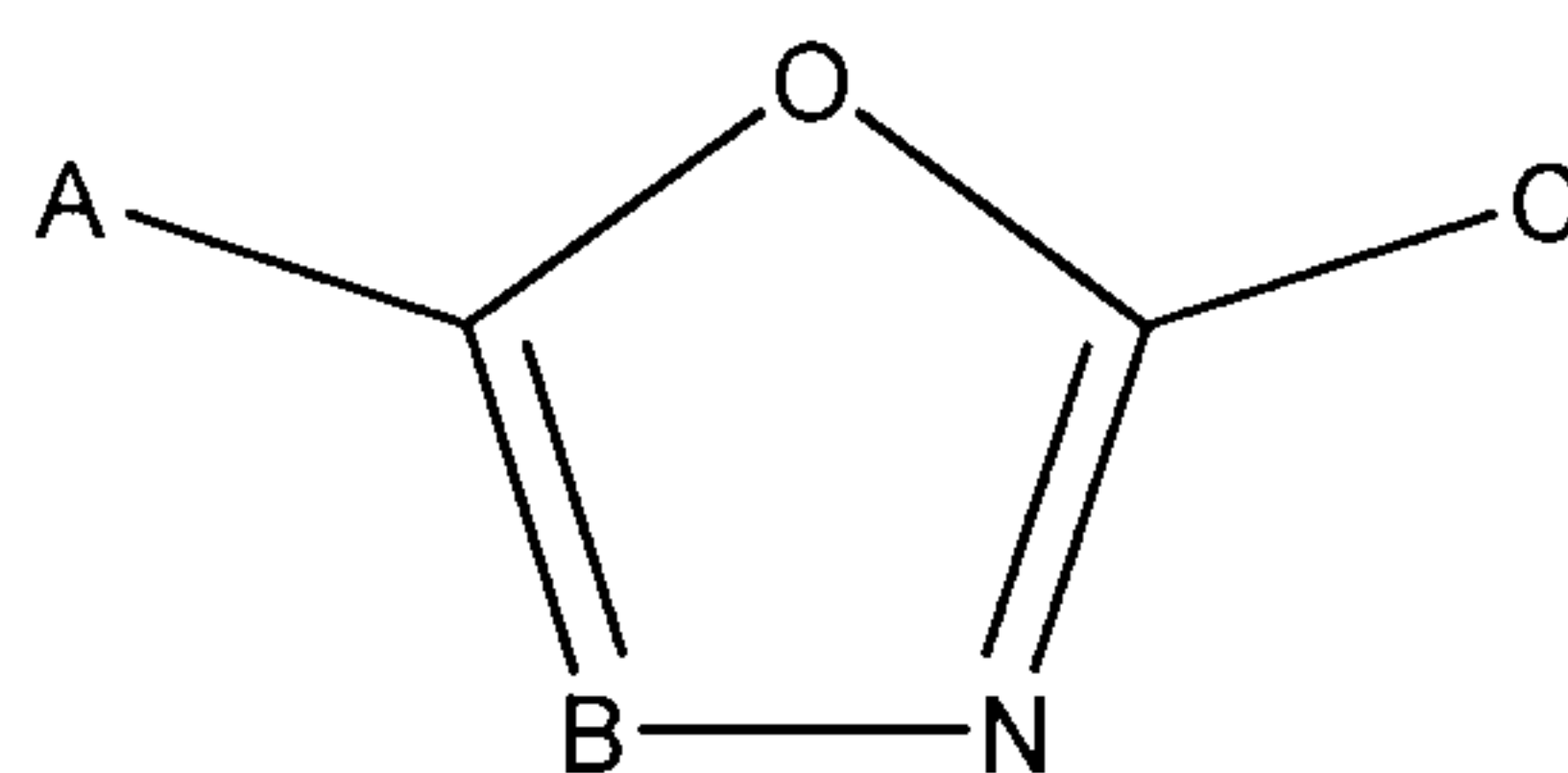
Formula I
