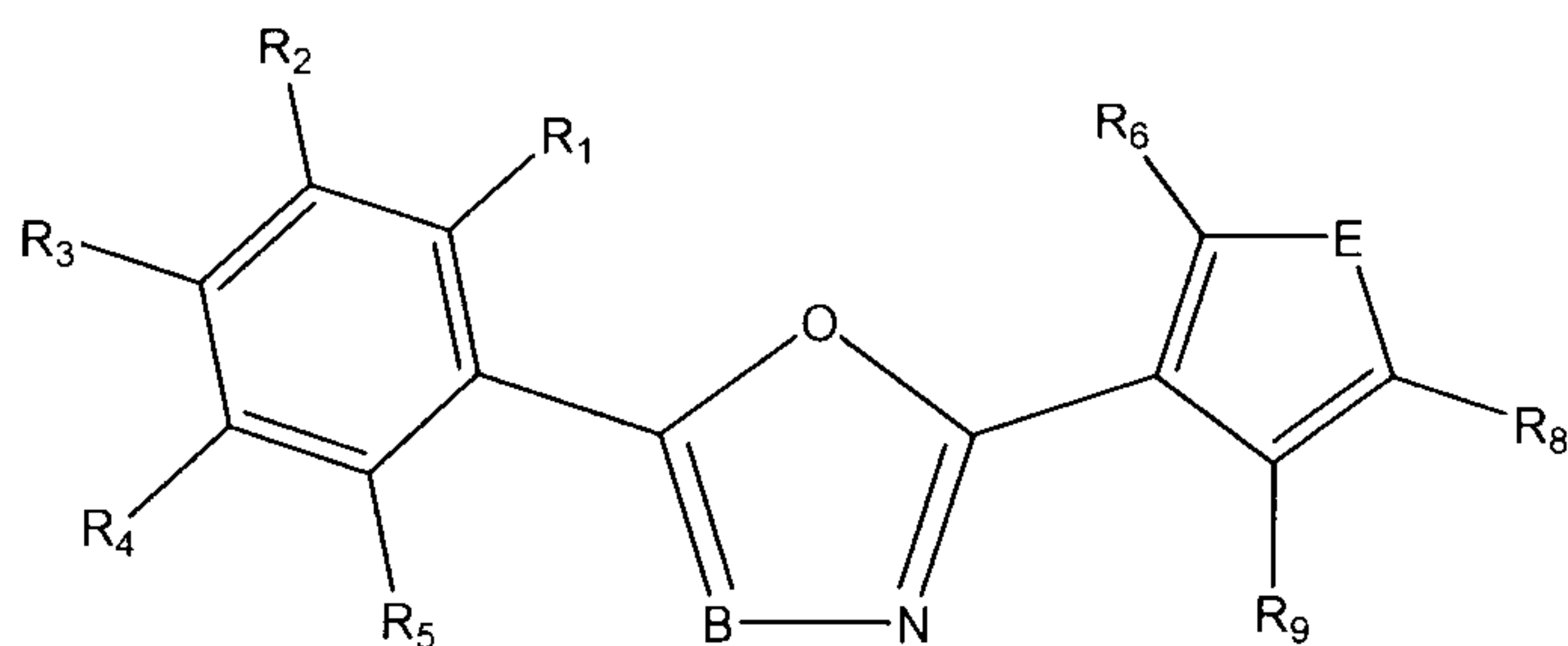
Formula Ib
