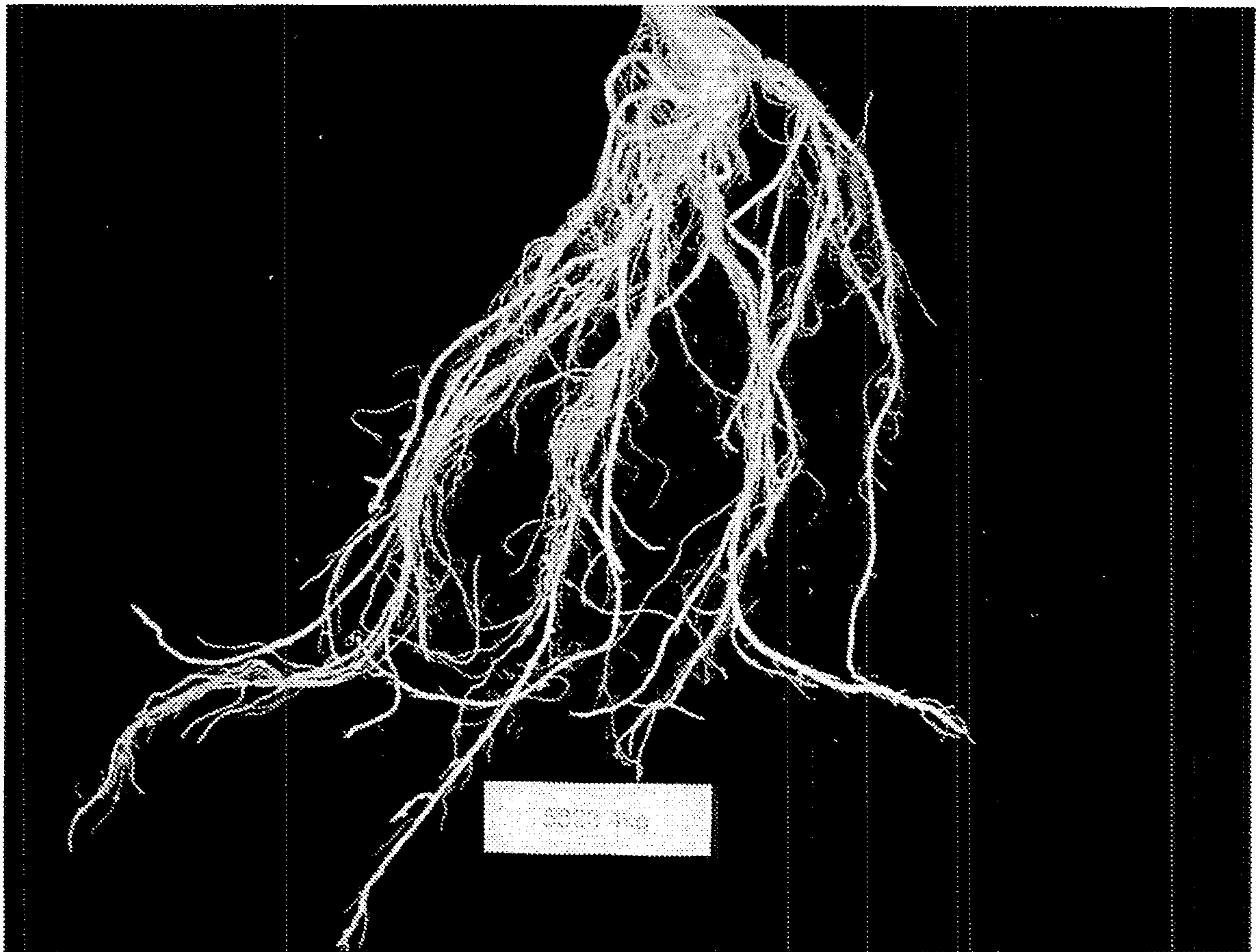
Figure 6: Roots from 4 kg/ha ai 5823 treated plants (Summer trial)
