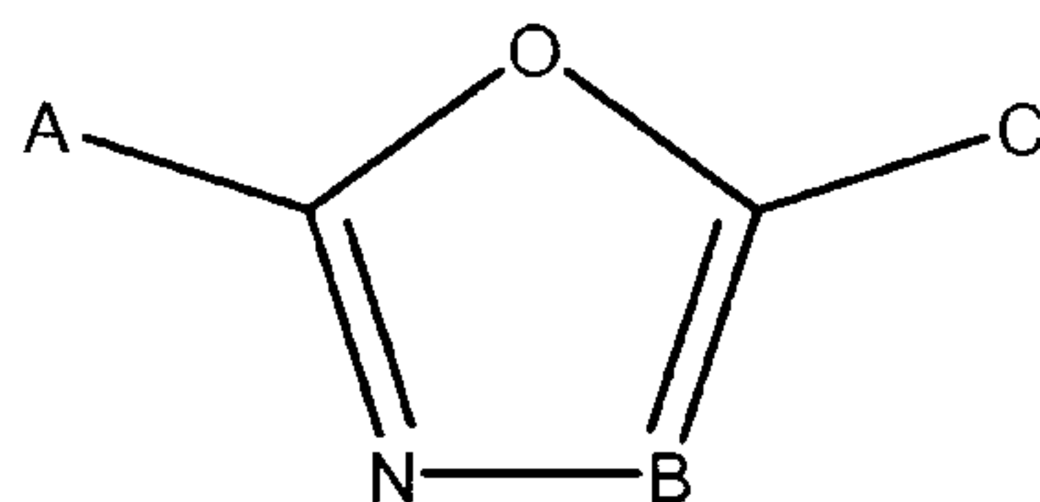
Formula II
