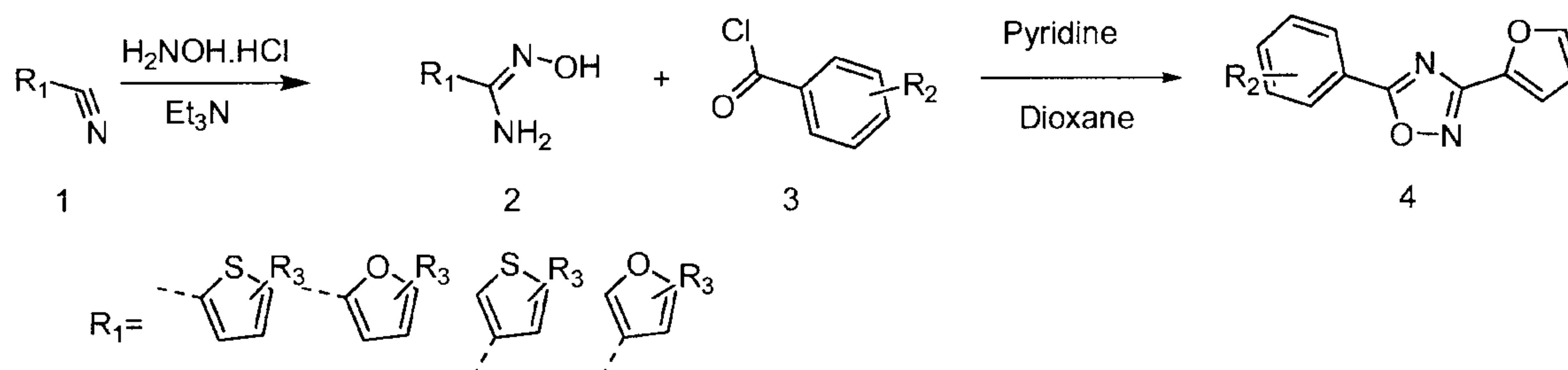
Scheme 5: Synthetic scheme to compounds of the Formula Va and Vb
