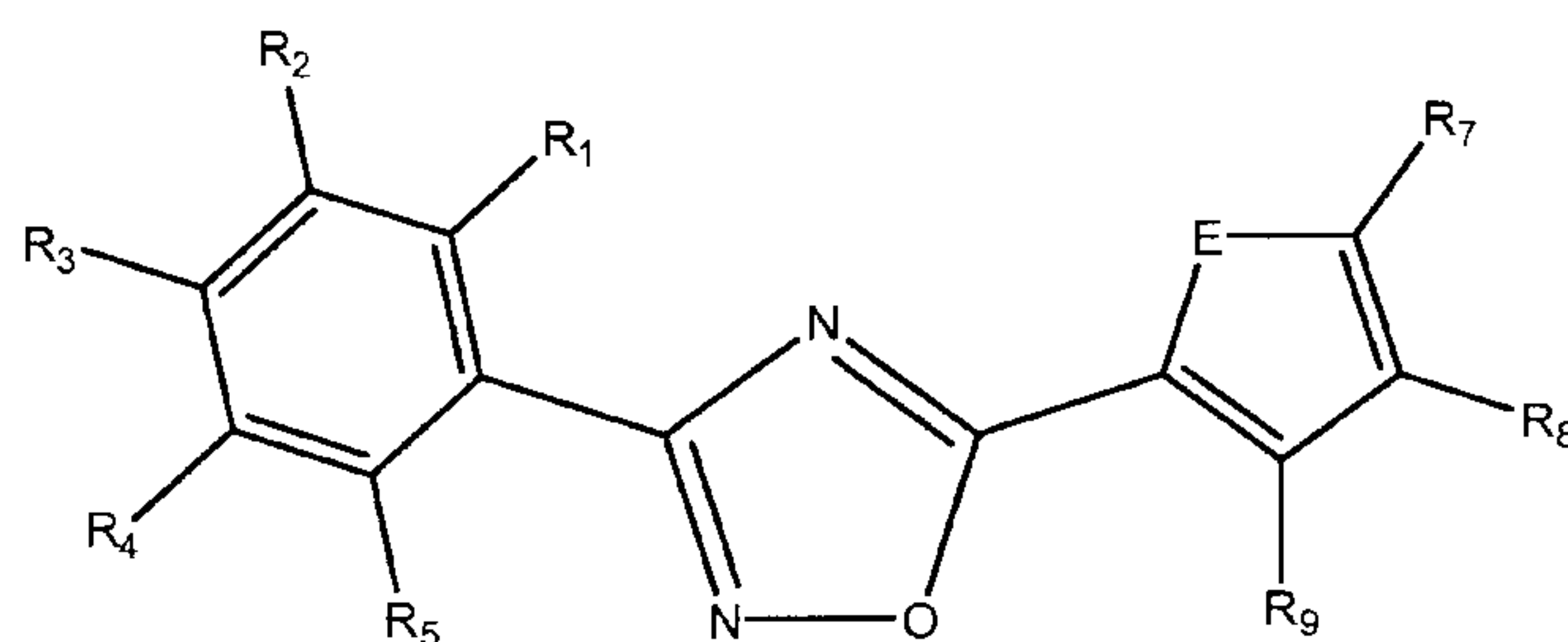
Formula IVa
