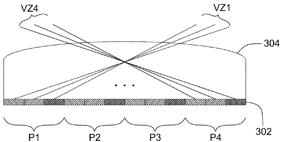
FIG. 3A(PRIOR ART)
