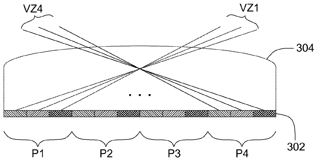
FIG. 4A(PRIOR ART)
