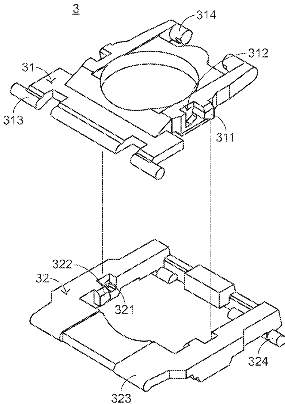
FIG.3 PRIOR ART
