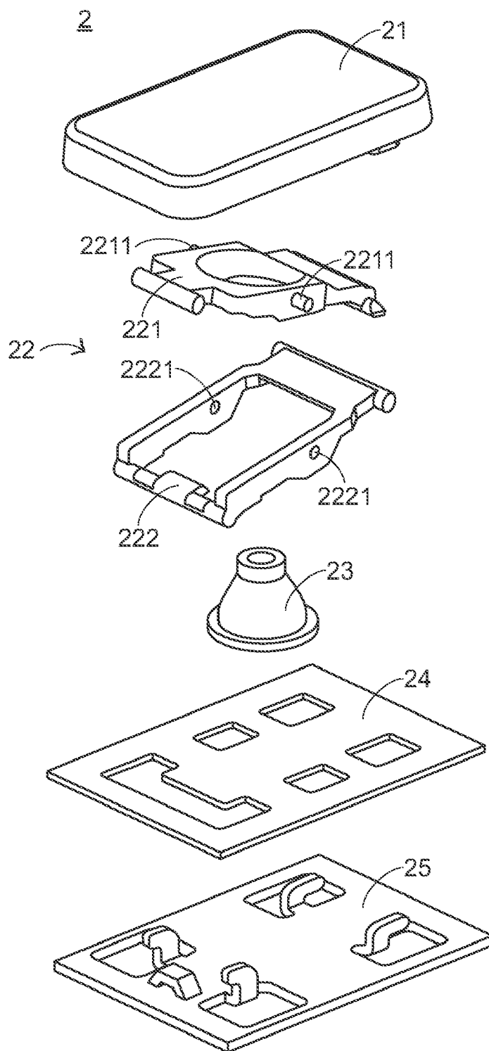
FIG.2 PRIOR ART
