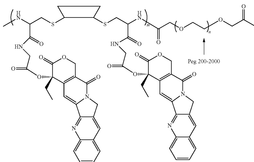
Scheme XXXXII
