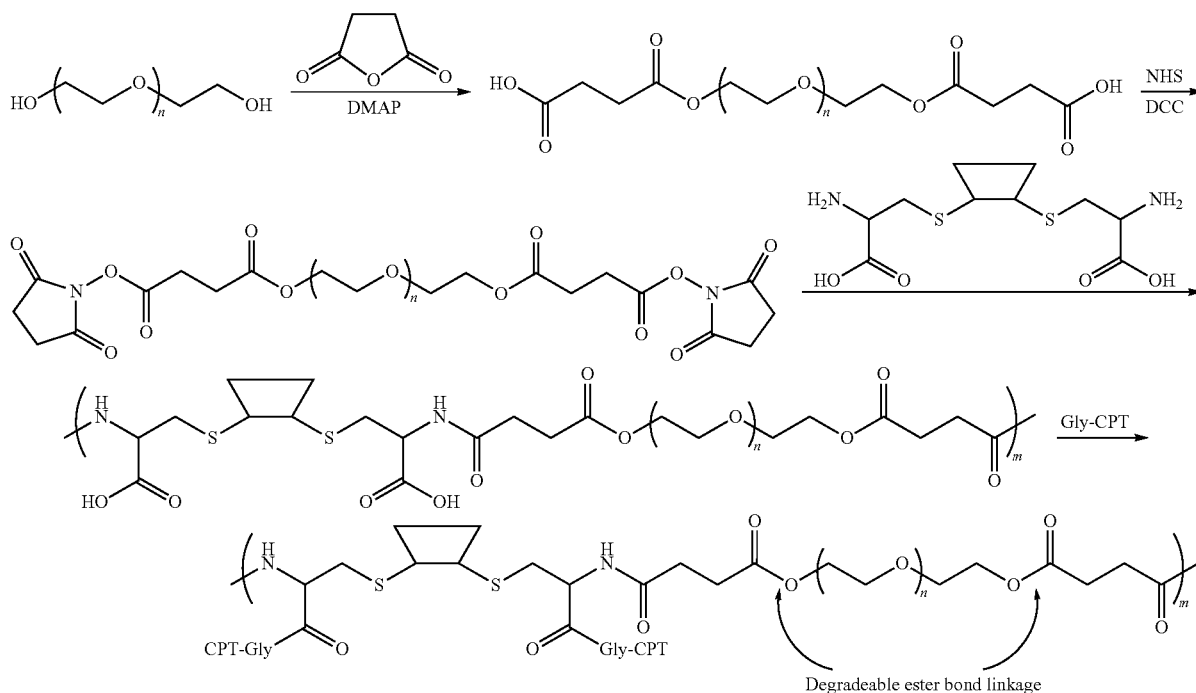
Scheme XIV
