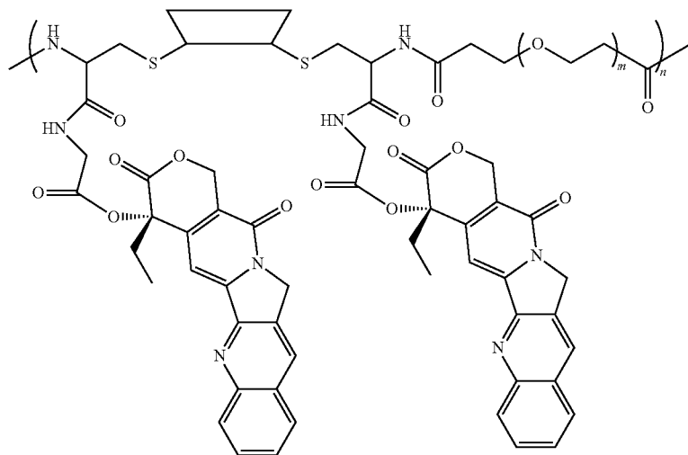
Scheme XXXXIII
