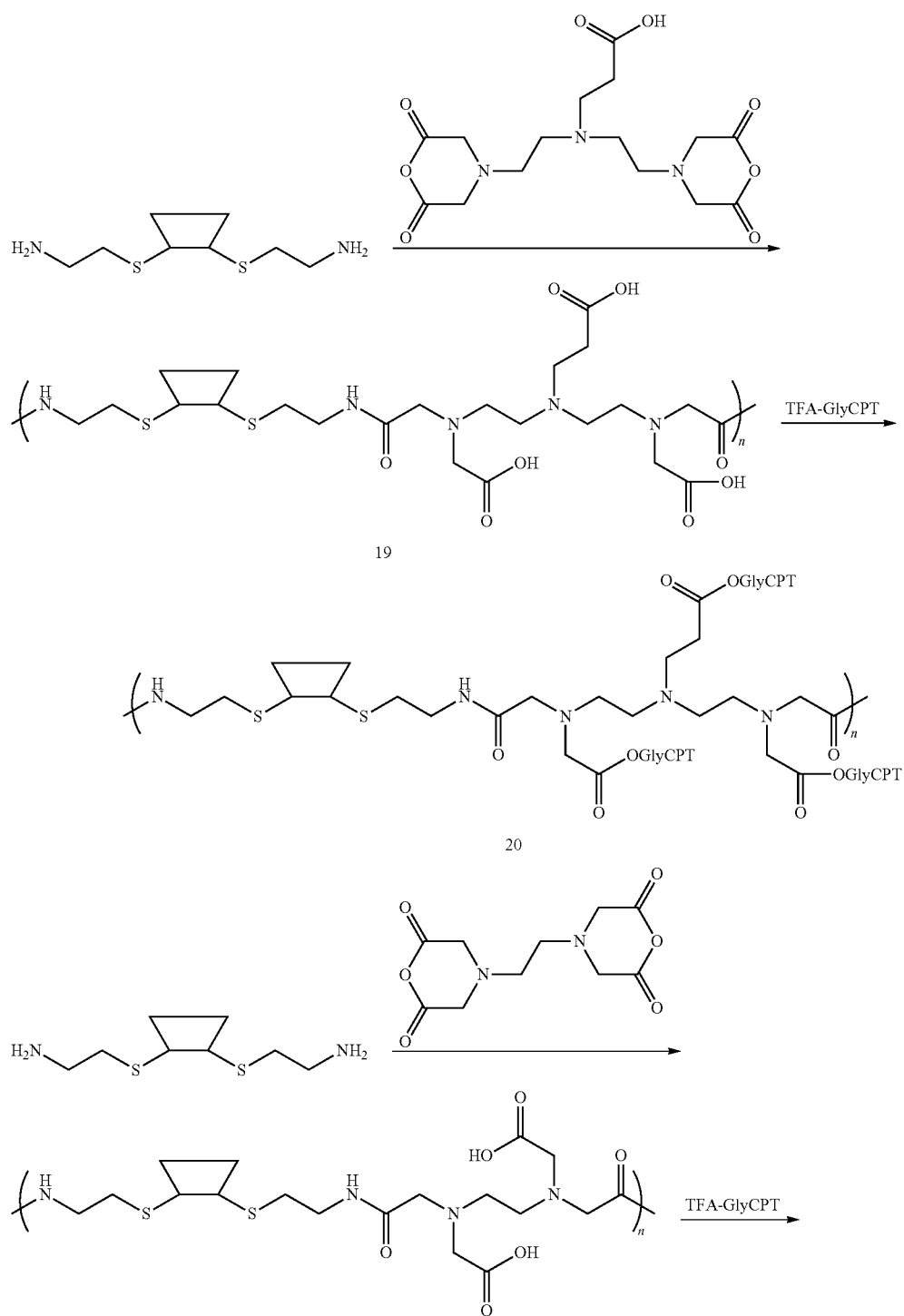
Scheme XXIX
