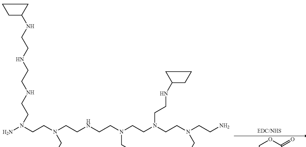
Scheme XXXXV
