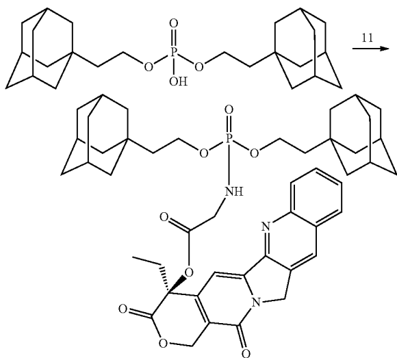
Scheme XXXXVIII
