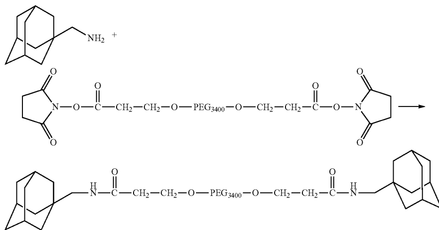
Scheme XXXXVI
