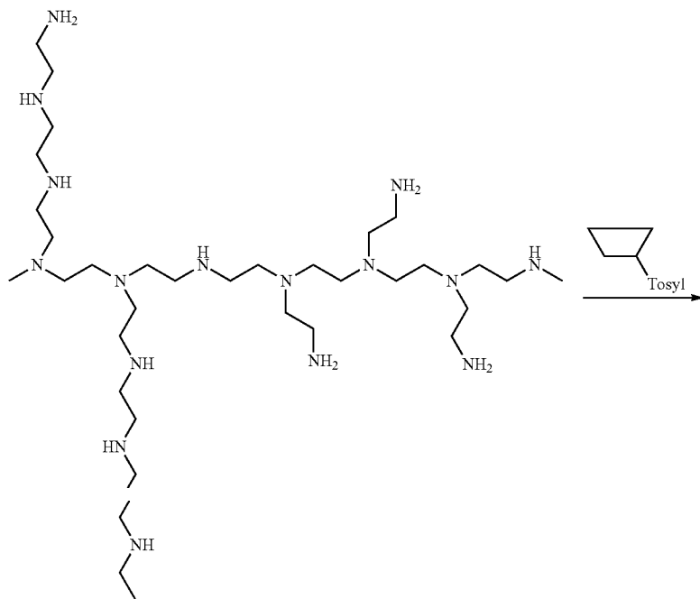
Scheme XXXXIV
