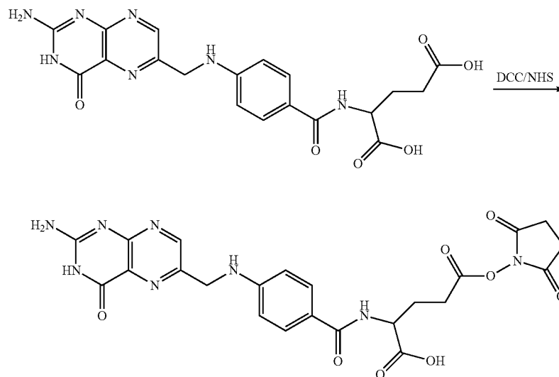
Scheme XXXXIX
