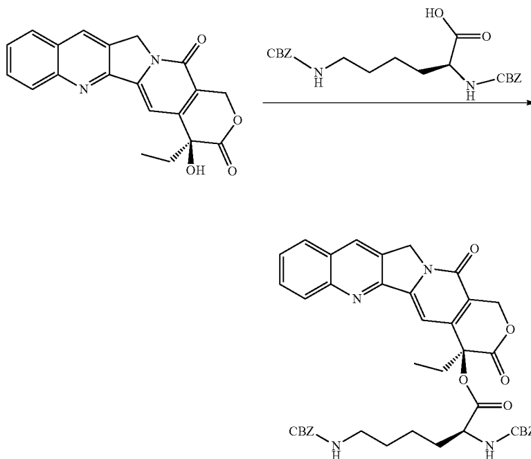
Scheme XXVII
