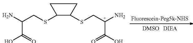
Scheme XXXX
