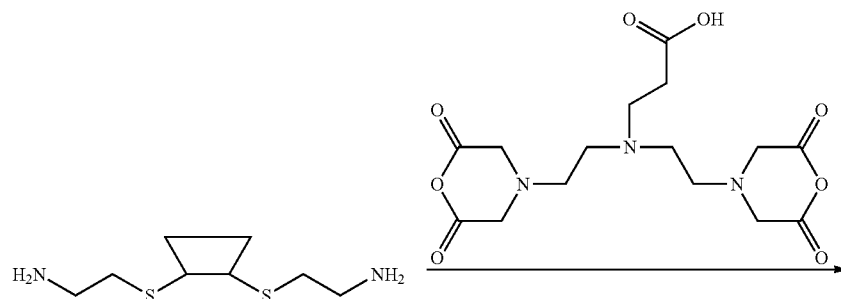
Scheme V
