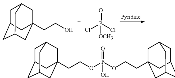
Scheme XXXXVII
