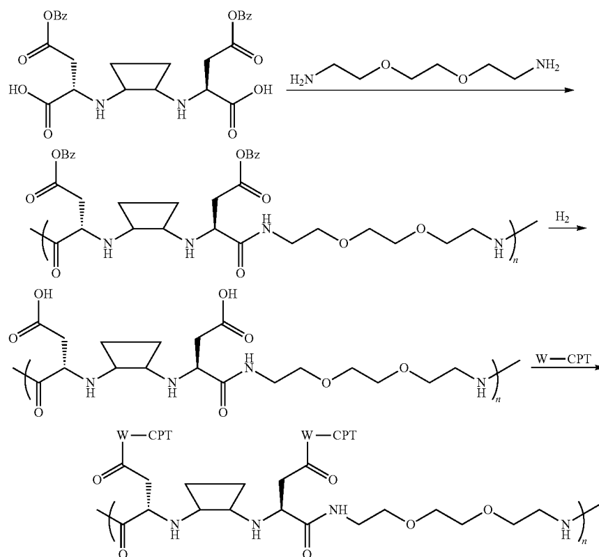
Scheme IV
