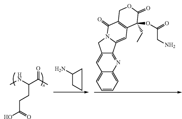
Scheme XXXVII
