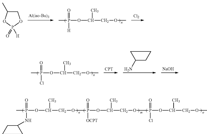
Scheme IX
