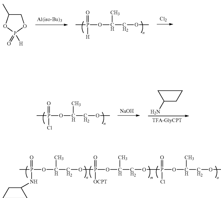
Scheme XXXIV
