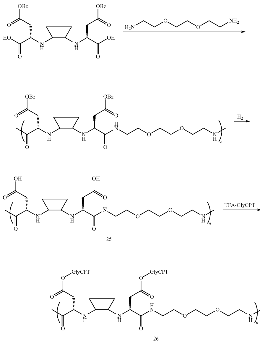
Scheme XXXI
