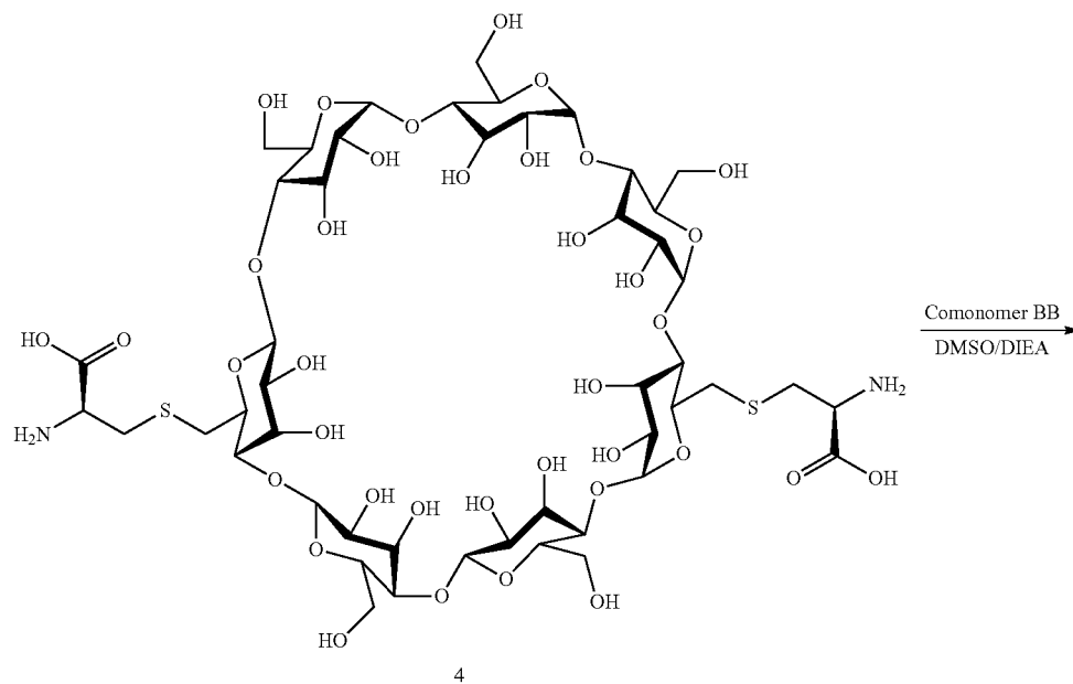
Scheme XXXVIIIb
