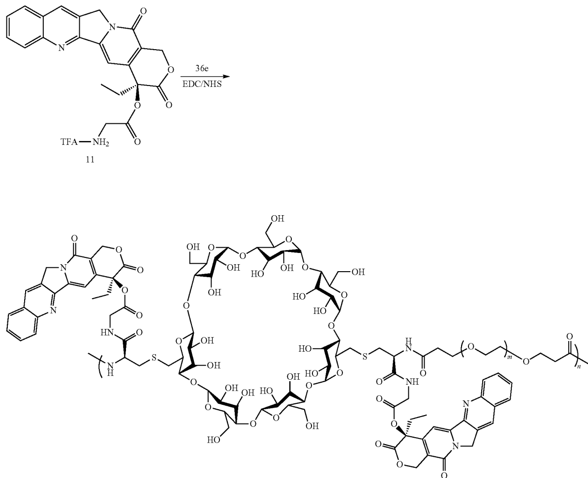
Scheme XXXIX
