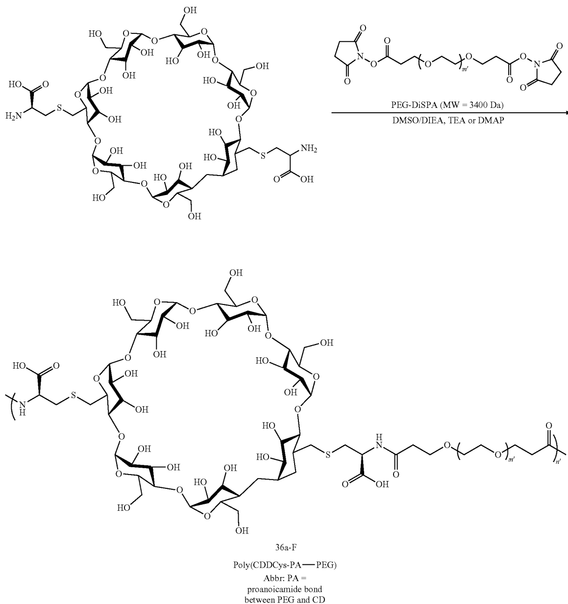
Scheme XXXVIIIa
