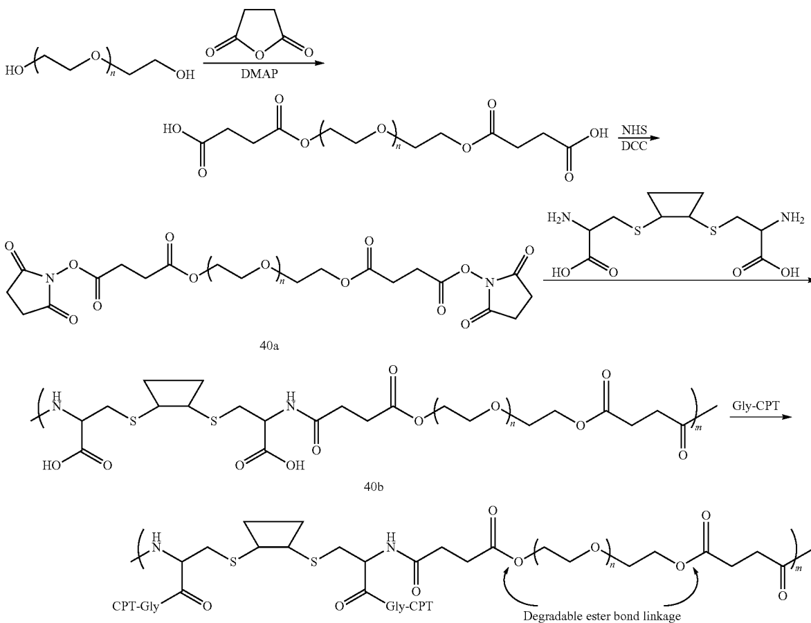
Scheme XXXXI
