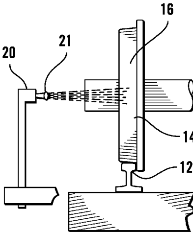
FIG. 2 (Prior Art)
