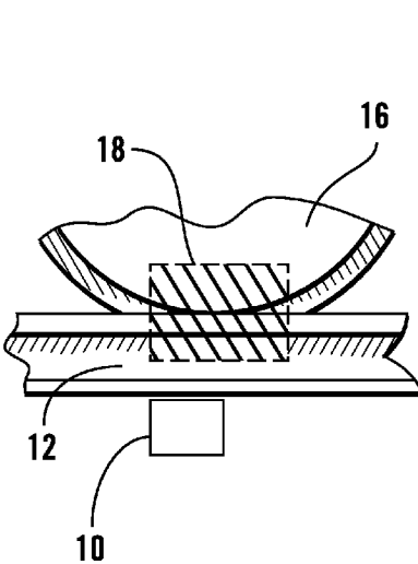
FIG. 3 (Prior Art)
