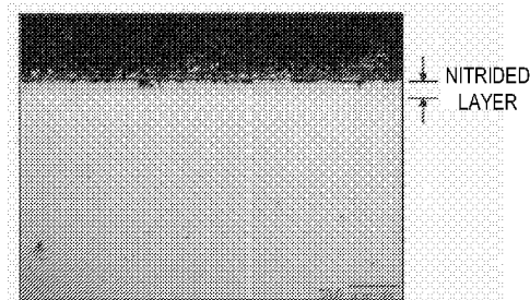
EXAMPLE (b) (NCF600: W/O GRINDING)
