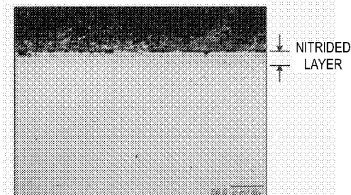
EXAMPLE (b)' (NCF601: W/O GRINDING)
