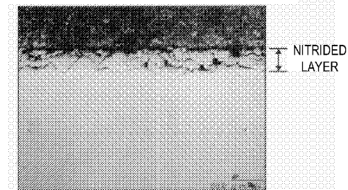
COMPARATIVE EXAMPLE (c) (NCF800: W/ GRINDING)
