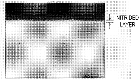
EXAMPLE (a) (NCF600: W/ GRINDING)
