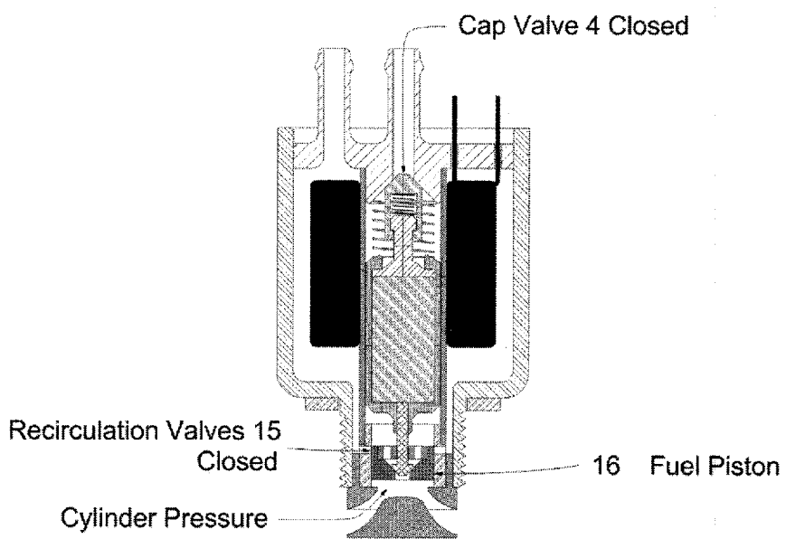
Figure 5 Cylinder Pressure Valve Closure
