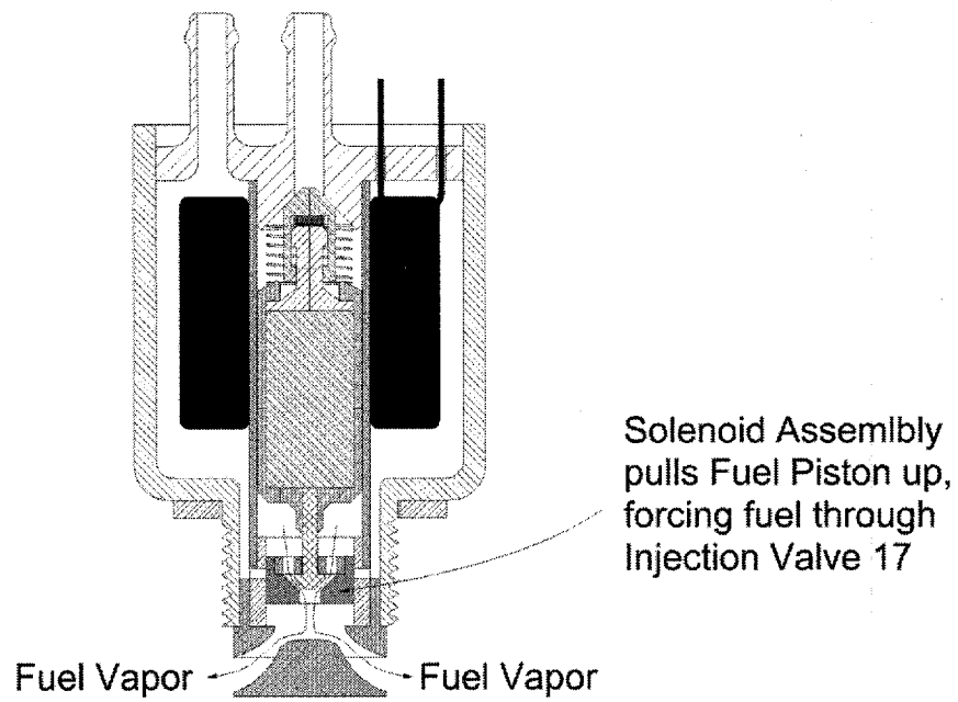
Figure 7 Fuel Injection
