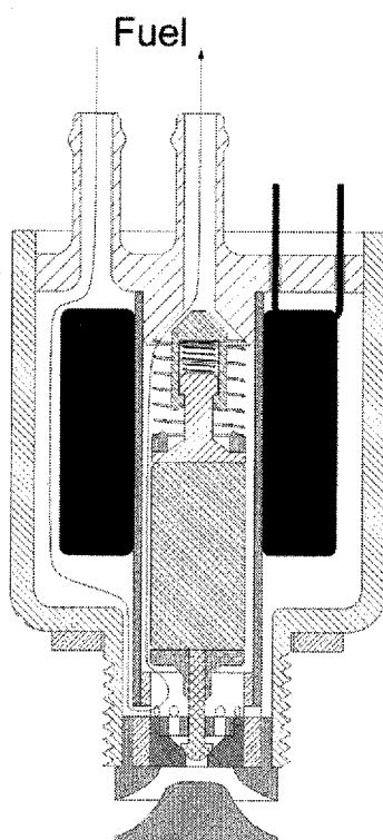
Figure 4 Recirculating Fuel Flow
