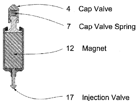
Figure 3A Solenoid Assembly
