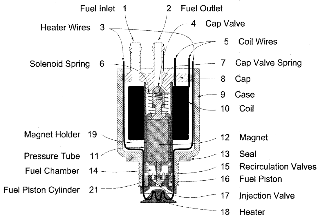
Figure 2 Injector Assembly
