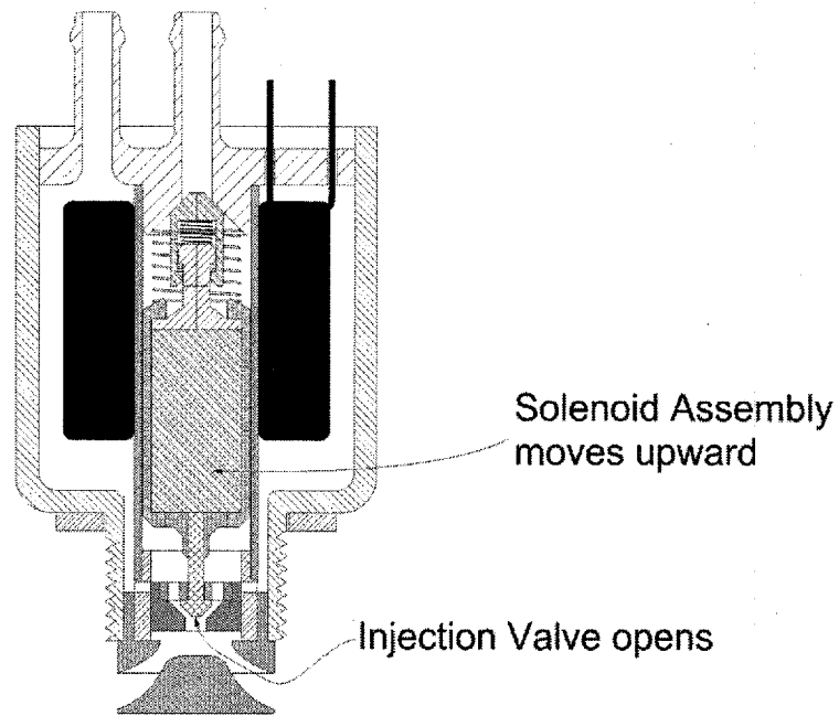
Figure 6 Solenoid Activation
