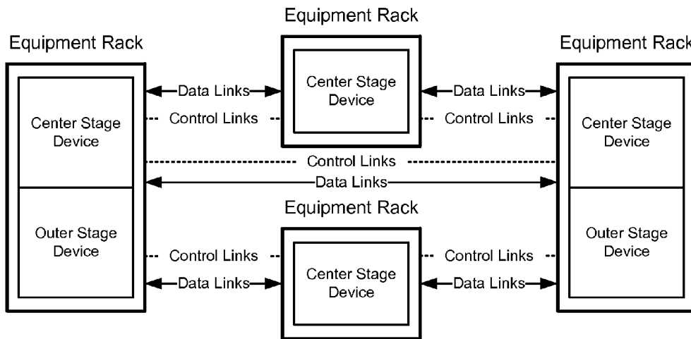
Fourth multi-chassis network switch (with modular center stage devices)
