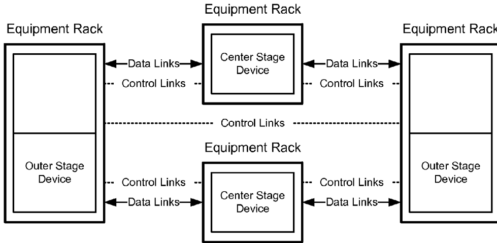
Third multi-chassis network switch (with modular center stage devices)
