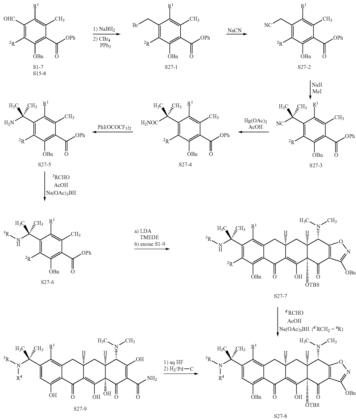
Scheme 27
