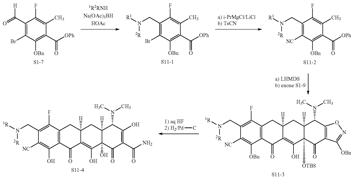
Scheme 11
