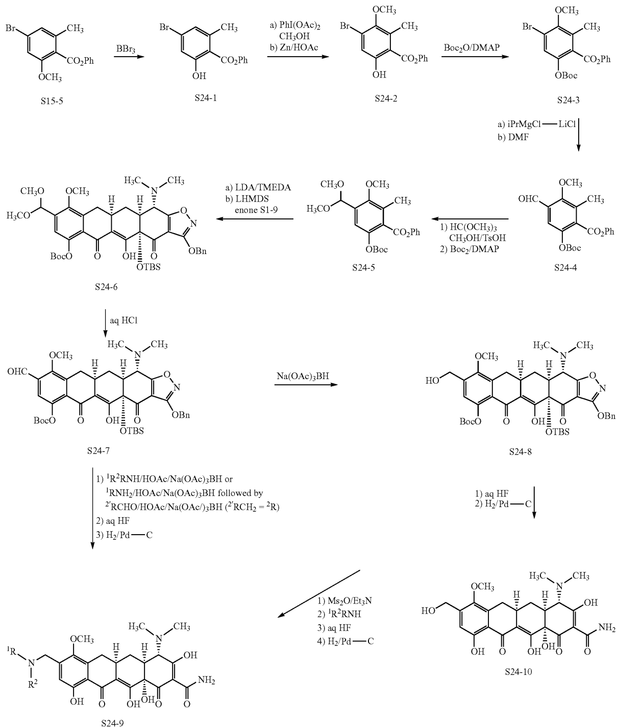
Scheme 24
