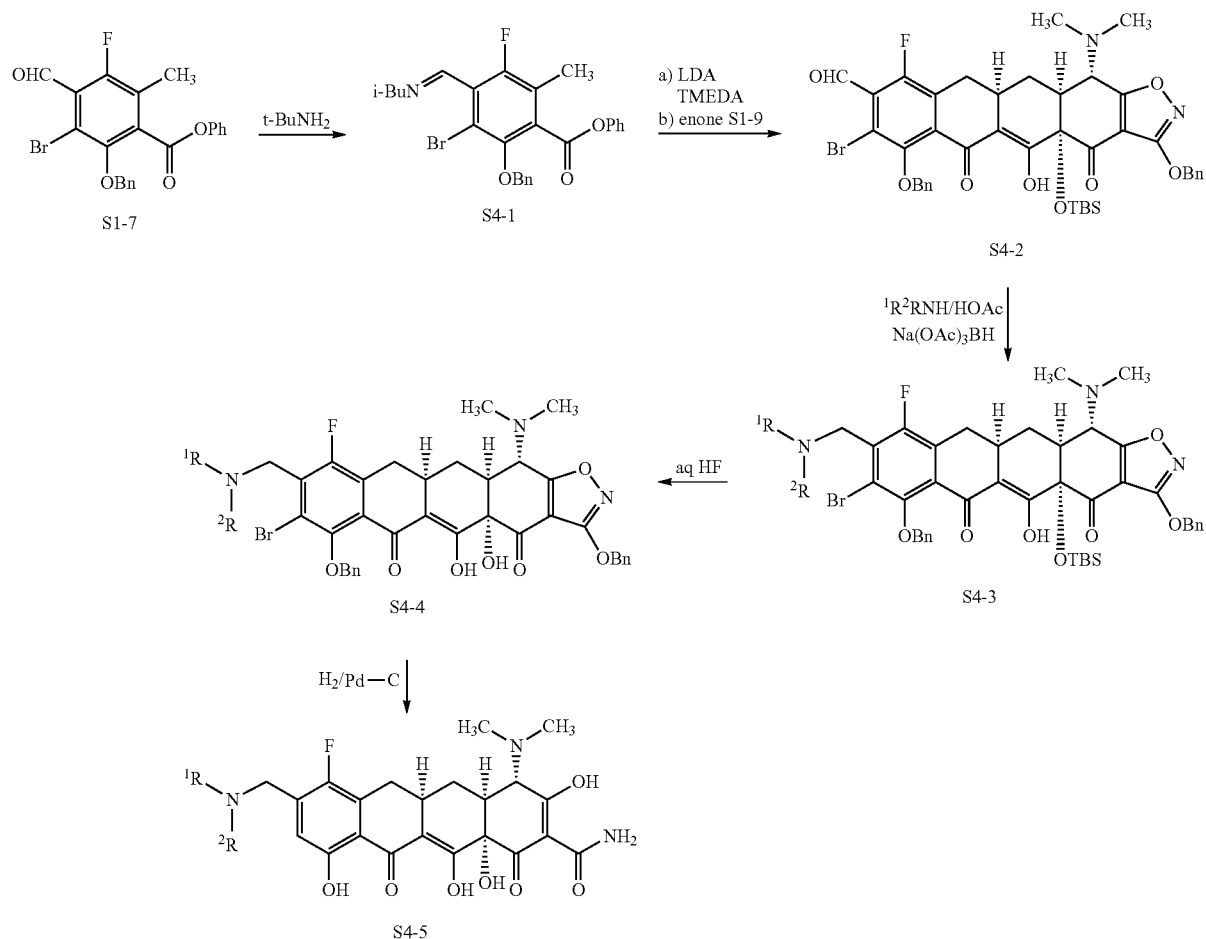
Scheme 4
