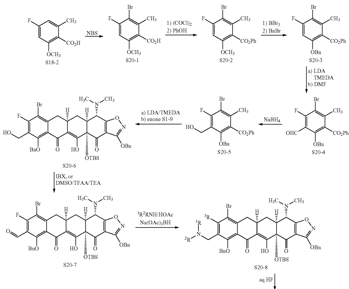
Scheme 20
