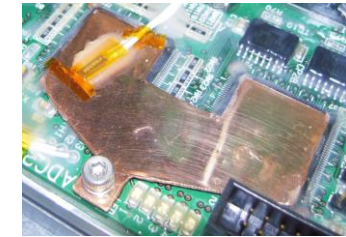
Example of a copper heat-path from an IC chip to a mechanical fastener.
