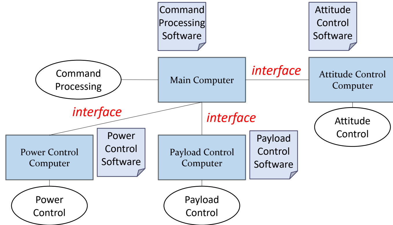
Distributed Computers
