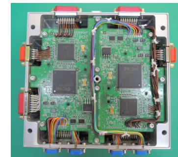
Example of a redundant computer unit, consisting of nominal and redundant computers.
