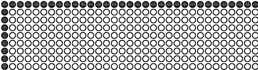
Prediction mode 2
