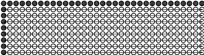
Prediction mode 1
