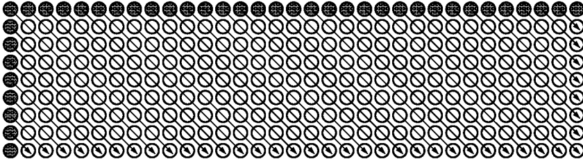
Prediction mode 4
