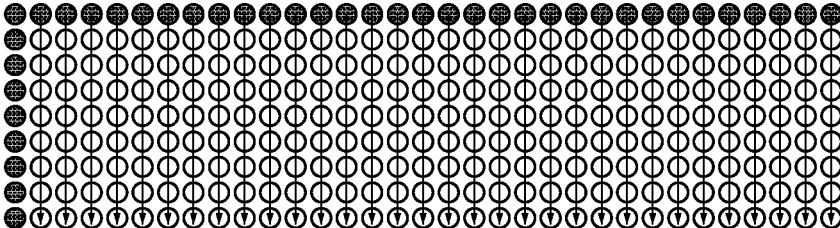
Prediction mode 0
