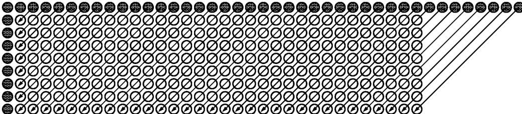
Prediction mode 3
