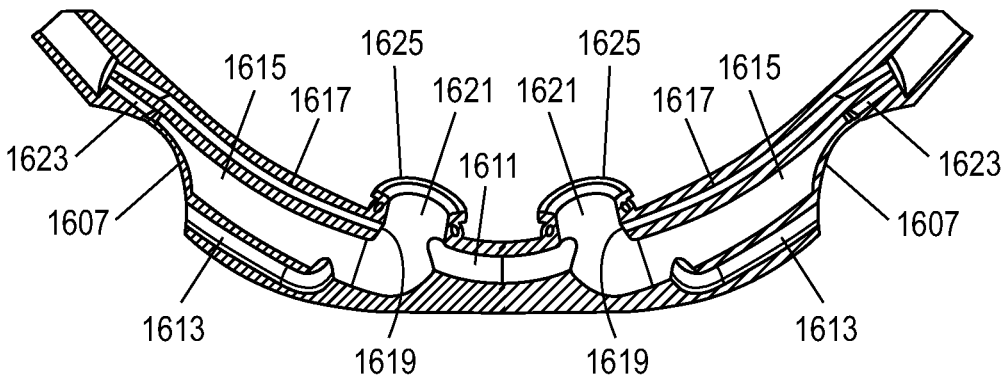
FIG. 18 SECTION E-E
