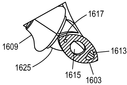
FIG. 19B SECTION F-F
