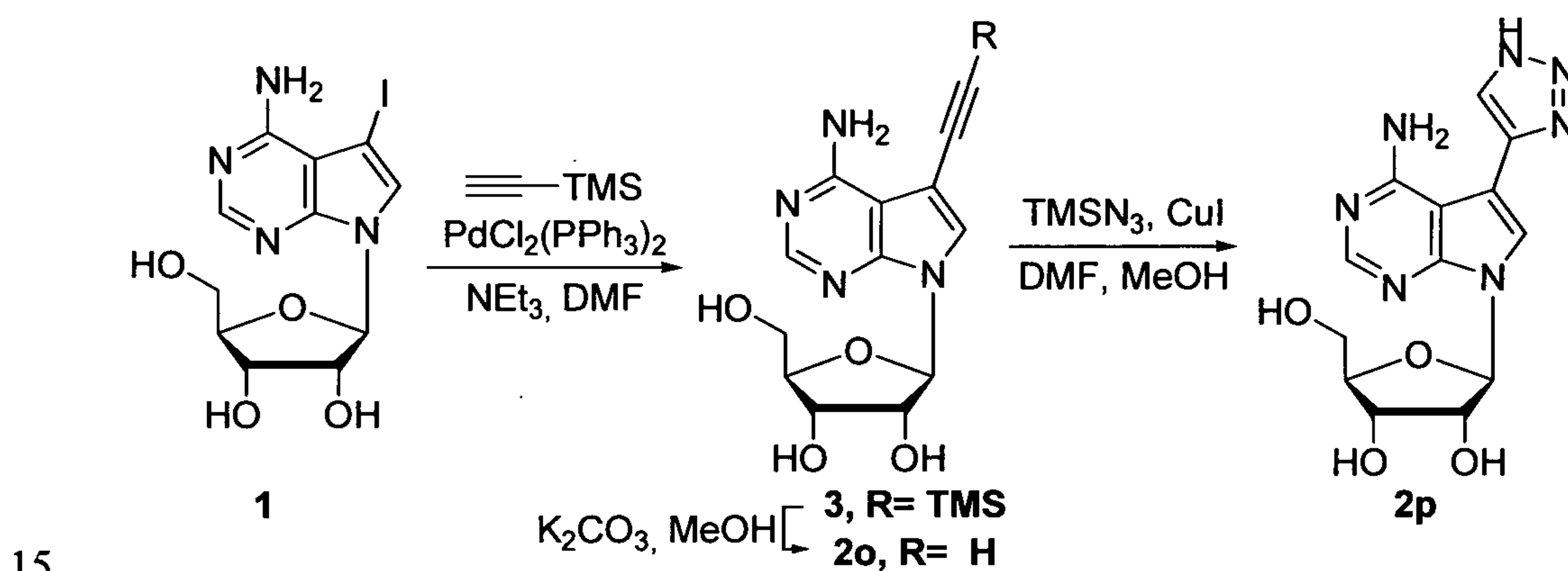
Scheme 2
