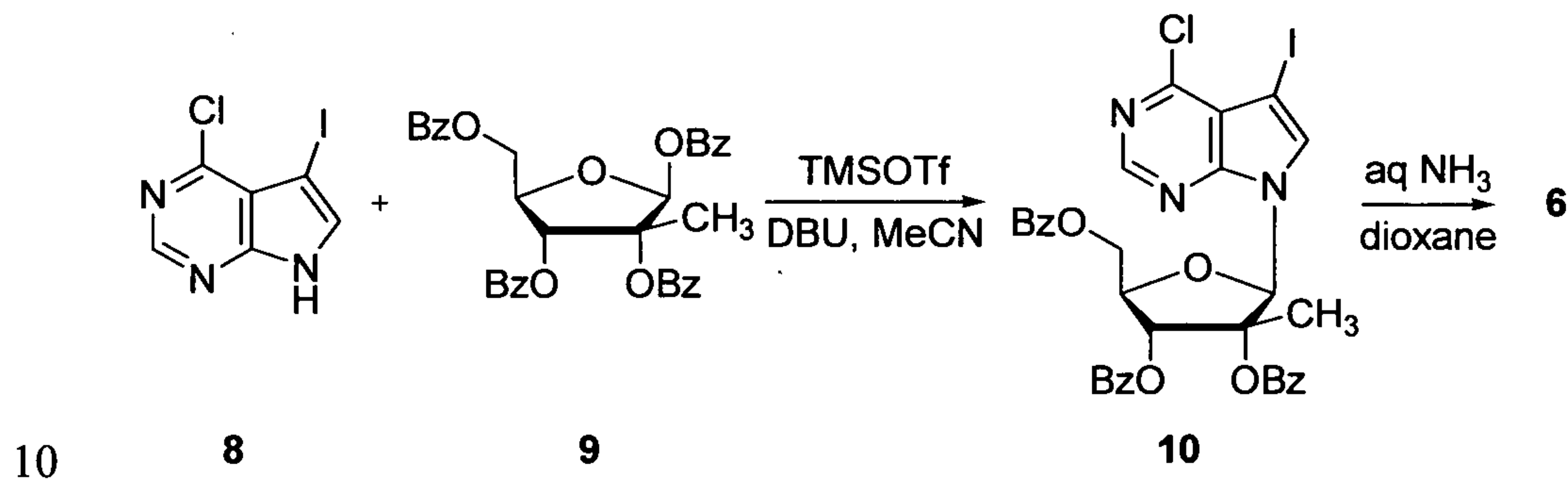
Scheme 5
