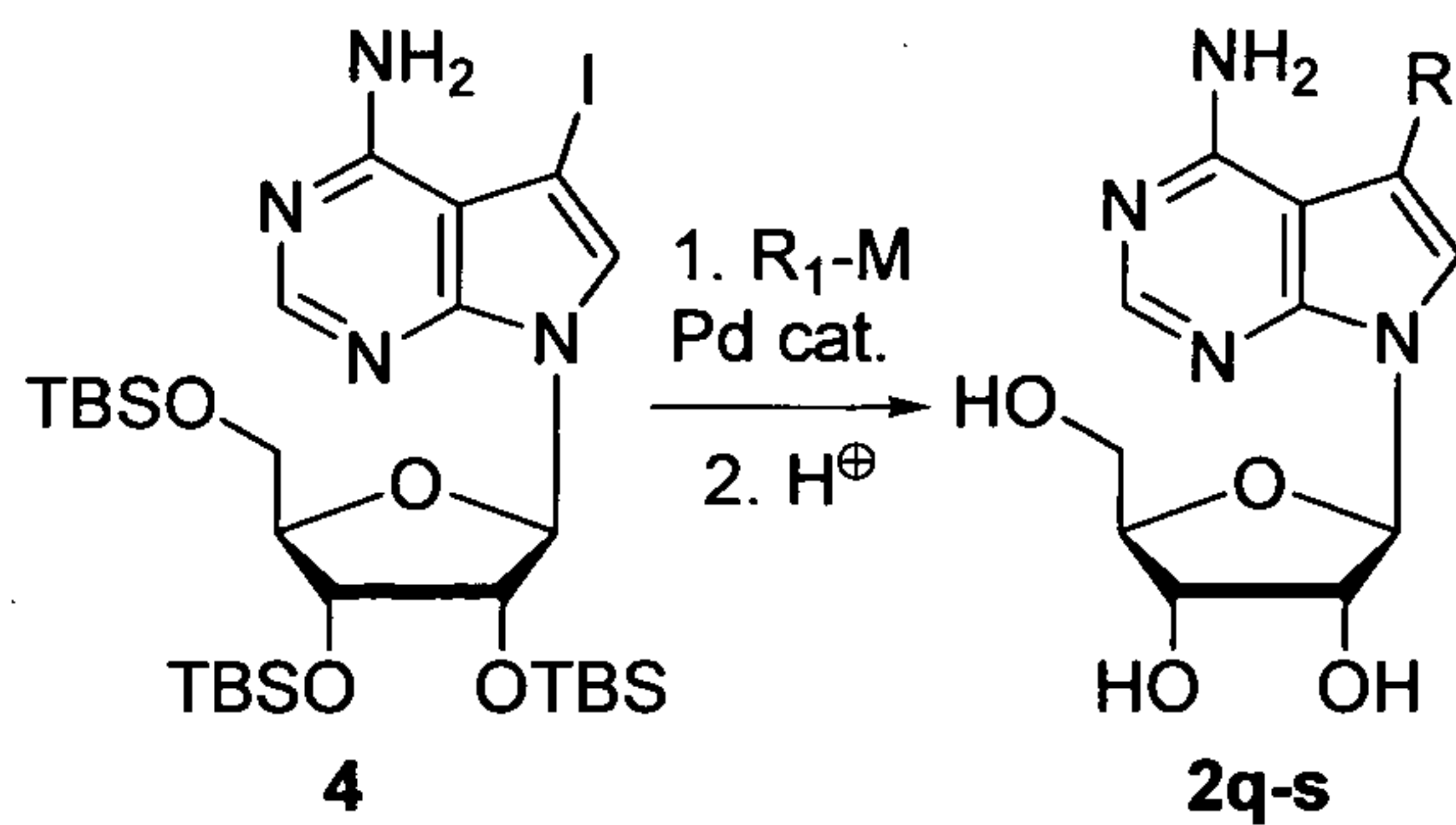
Scheme 3
