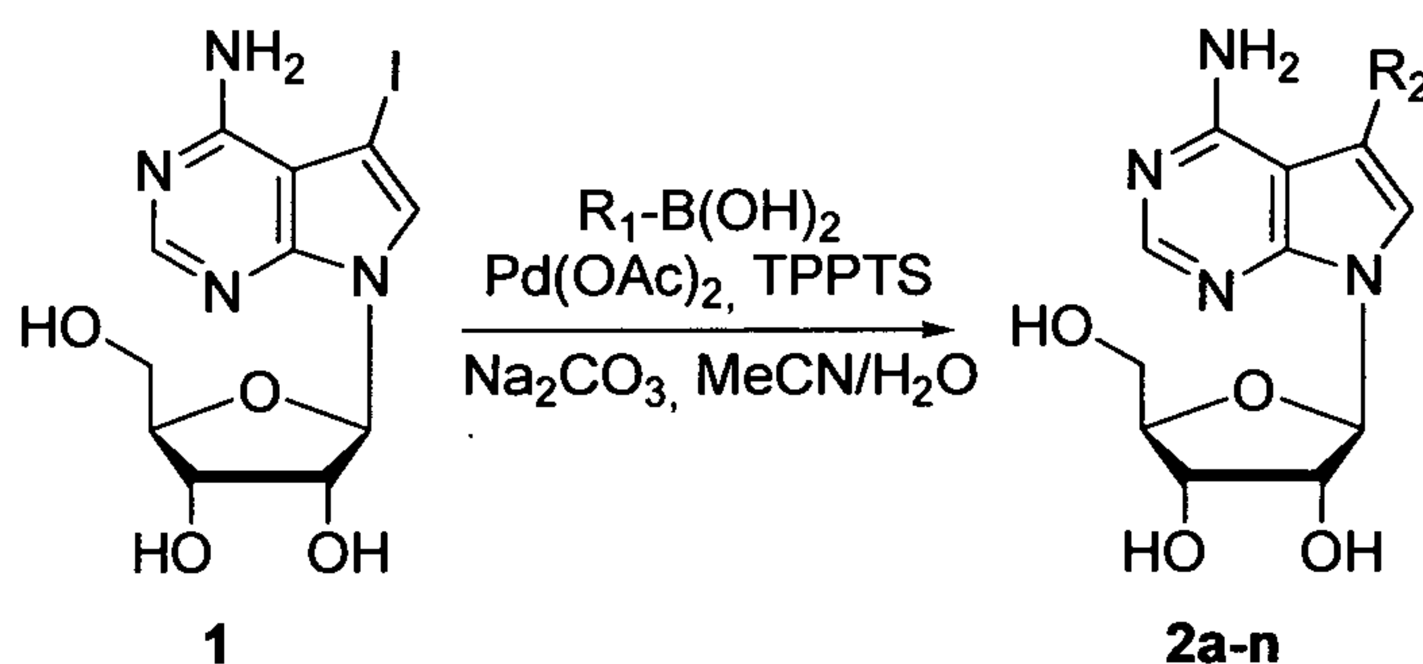
Scheme 1
