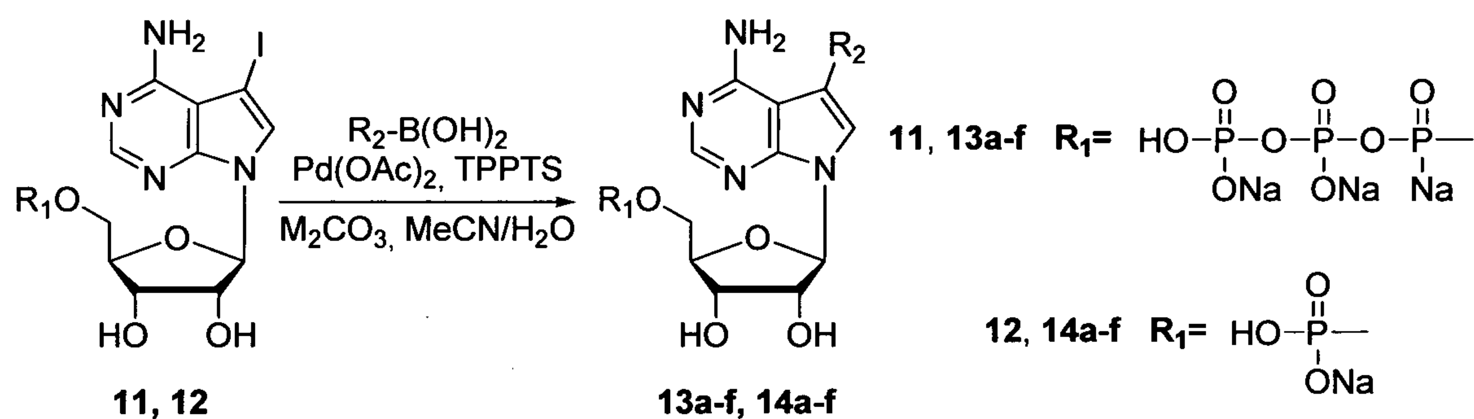
Scheme 6
