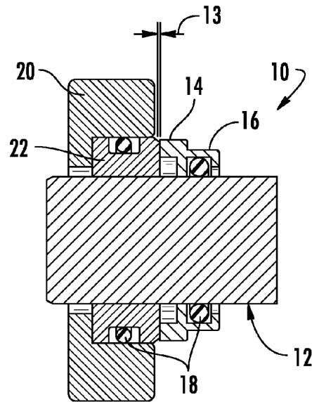
FIG. 1 (PRIOR ART)
