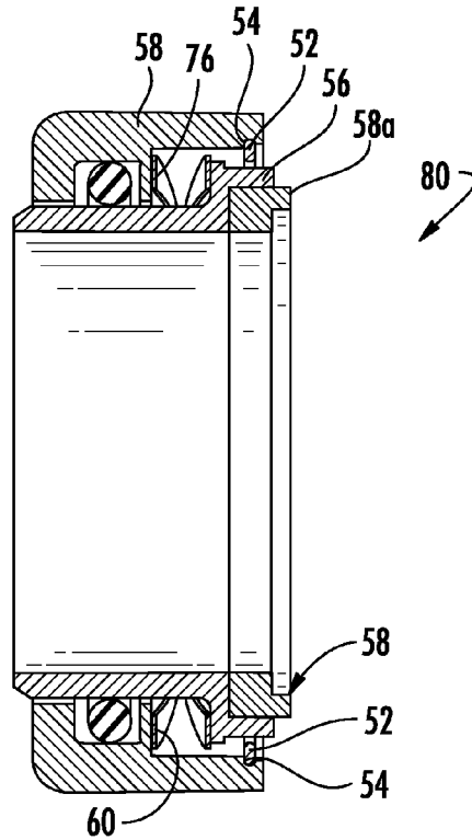
FIG. 3 (PRIOR ART)
