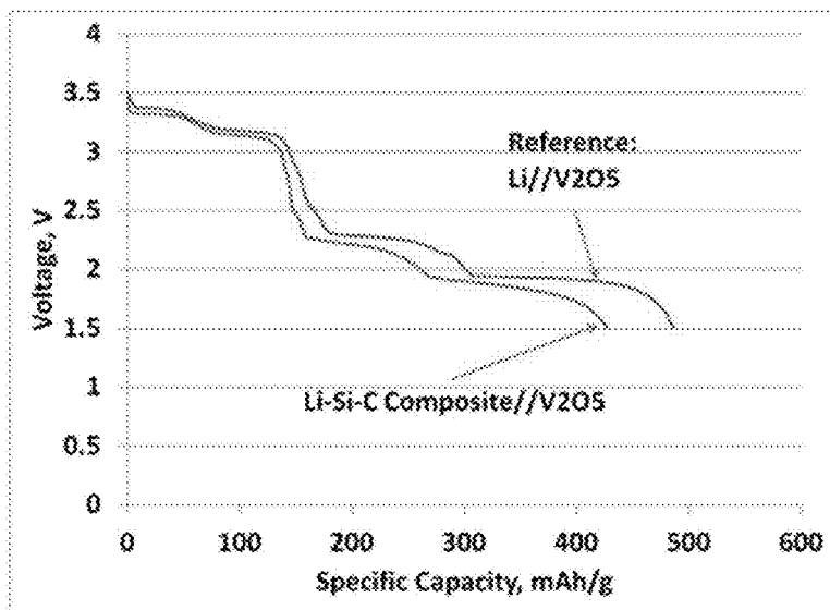
Figure 20. Discharge of primed cell (blue): Li-Si-C/V 2 O 5 composite. A Li/V 2 O 5 cell is shown as a reference (red).
