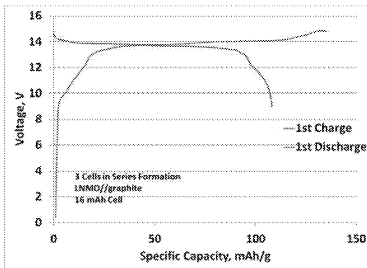
Electrochemical Performance of Three-Cell Stack.
