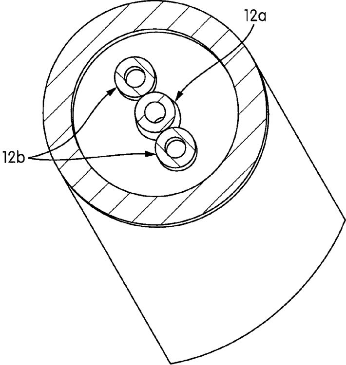
DETAIL D FIG. 3
