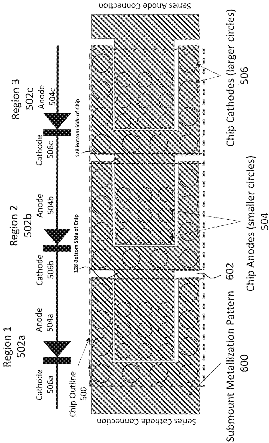
Figure 6 (Bottom side of chip)
