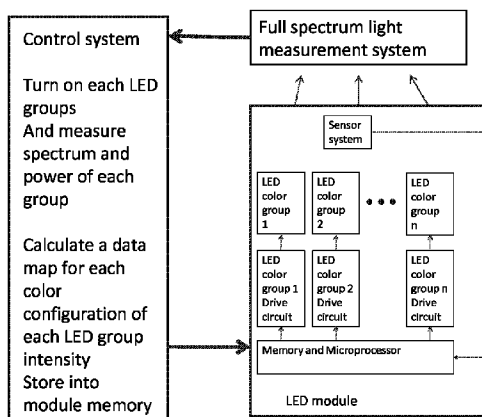
LED module tuning and control algorithm
