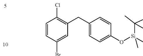
[4-(5-bromo-2-chloro-benzyl)-phenoxy]-tert-butyl-dimethyl-silane
