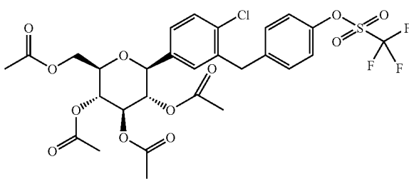
1-chloro-4-(2,3,4,6-tetra-O-acetyl-β-D-glucopyranos-1-yl)-2-[4-(trifluoromethylsulphonyloxy)-benzyl]-benzene
