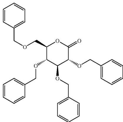
2,3,4,6-Tetra-O-benzyl-D-glucopyranone
