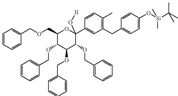
1-(2,3,4,6-Tetra-O-benzyl-1-hydroxy-D-glucopyranos-1-yl)-3-[4-(tert-butyl-dimethyl-silyloxy)-benzyl]-4-methyl-benzene
