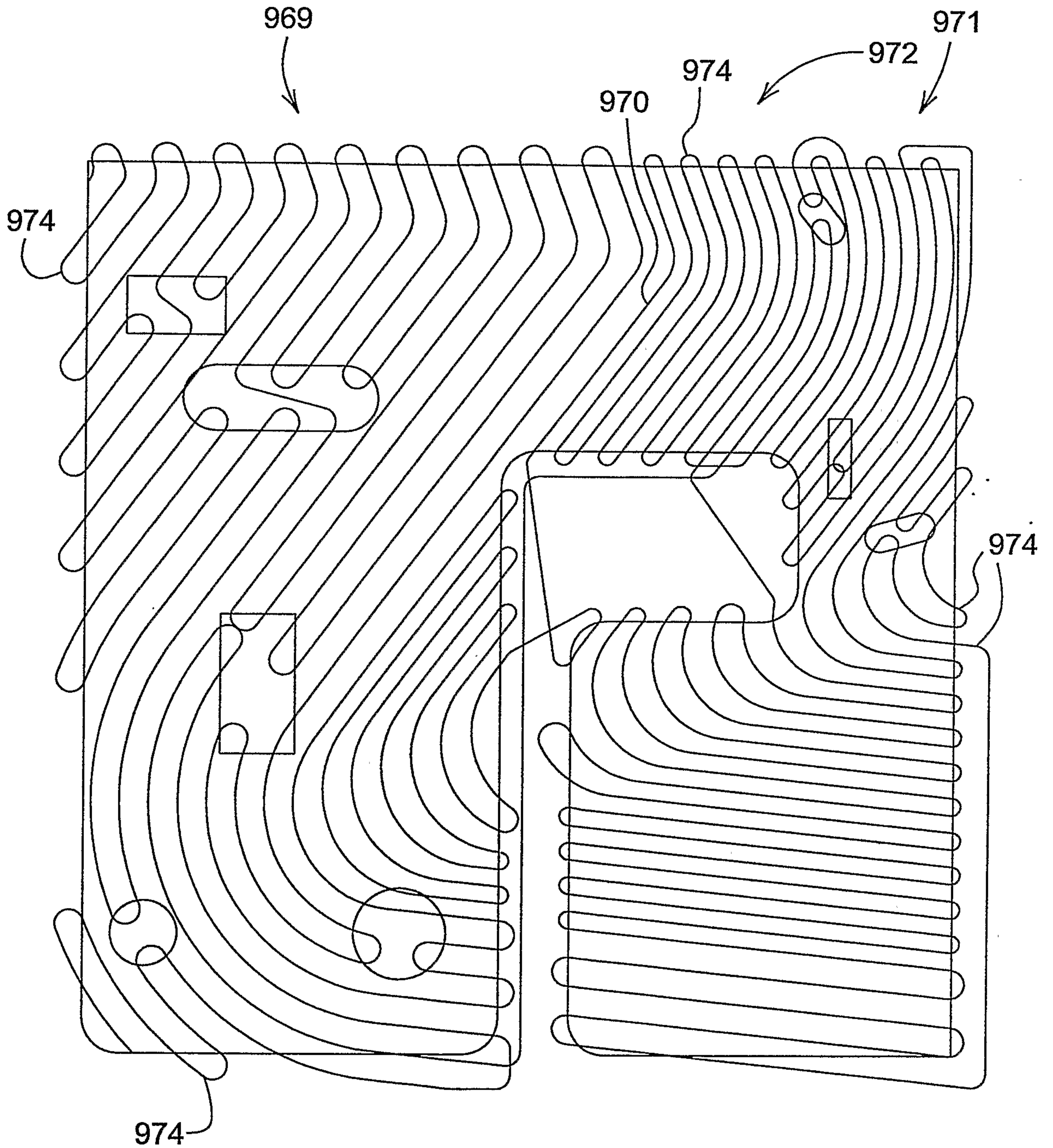
Fig. 21C Coverage Solution
