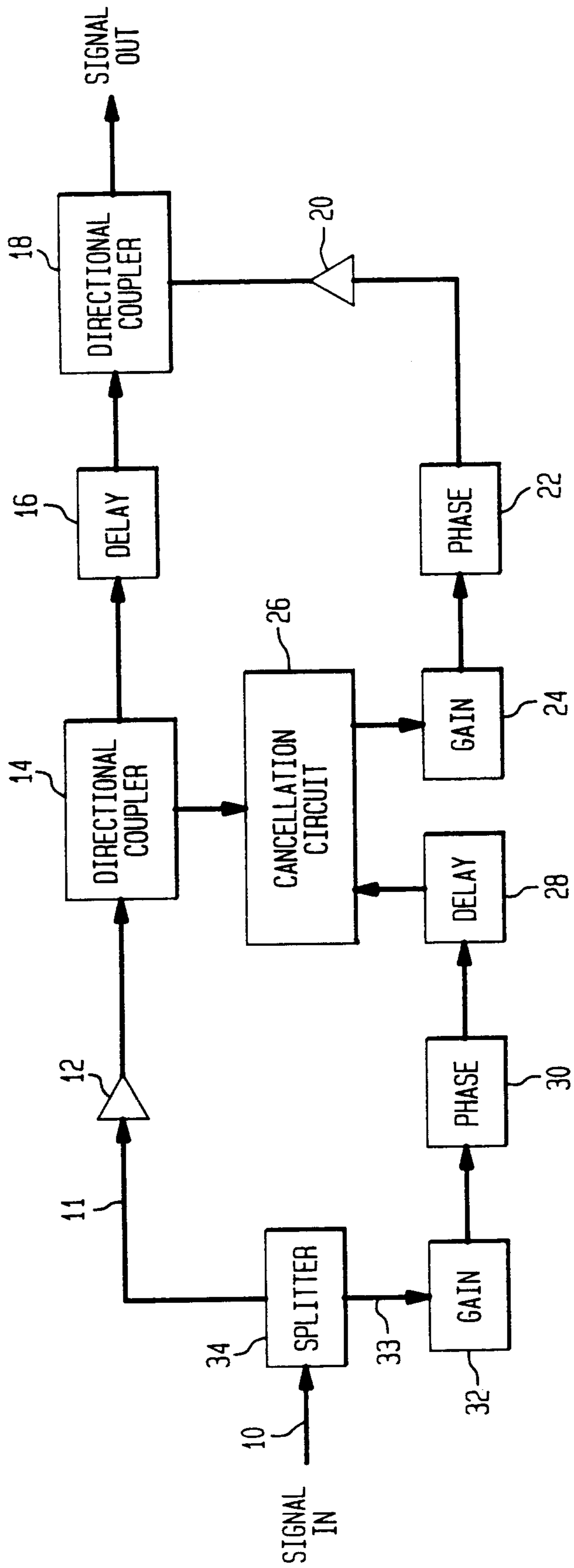
FIG. 1 (PRIOR ART)
