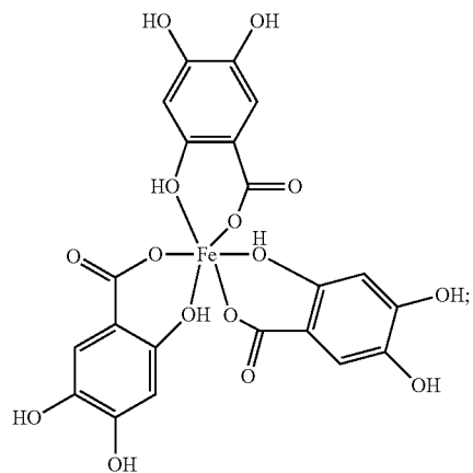
Formula VIII
