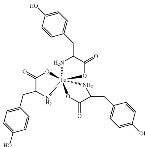
Formula VIII
