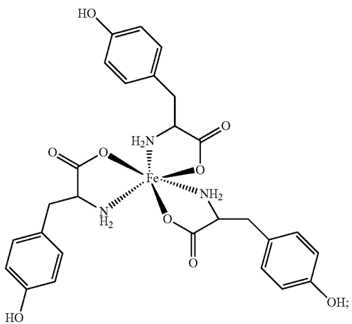
Formula VIII
