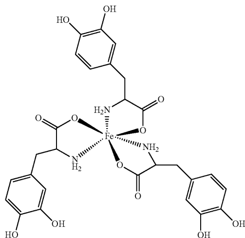
Formula VII
