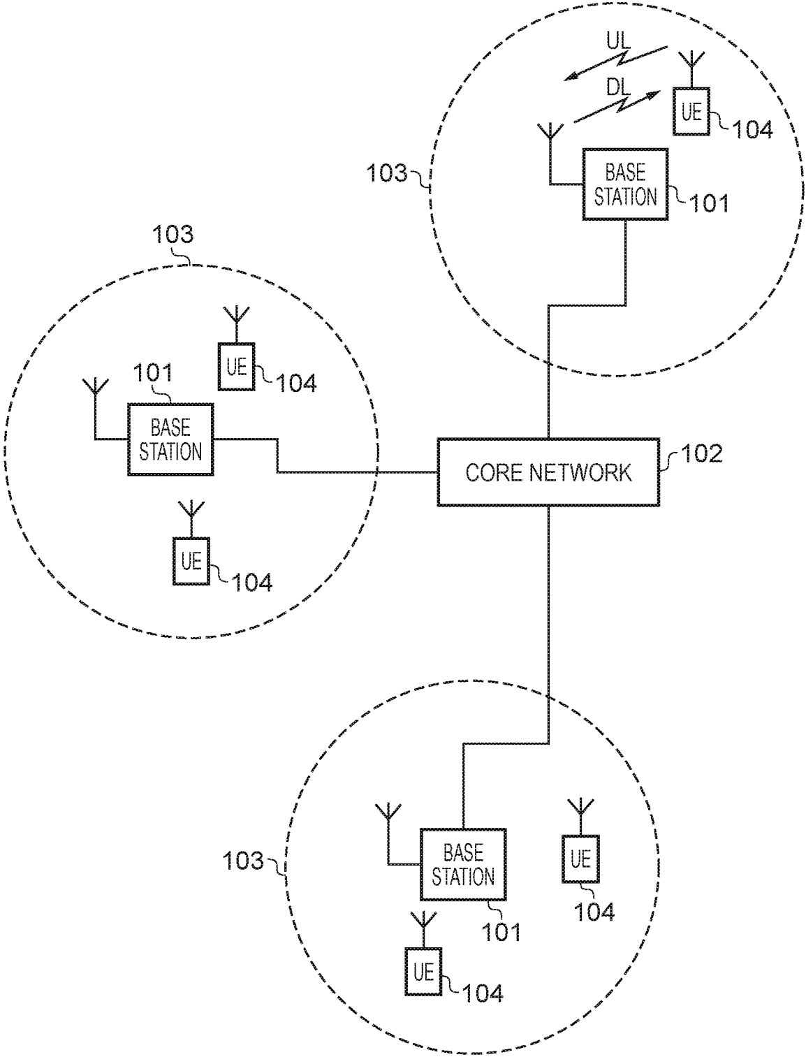
FIG. 1 PRIOR ART
