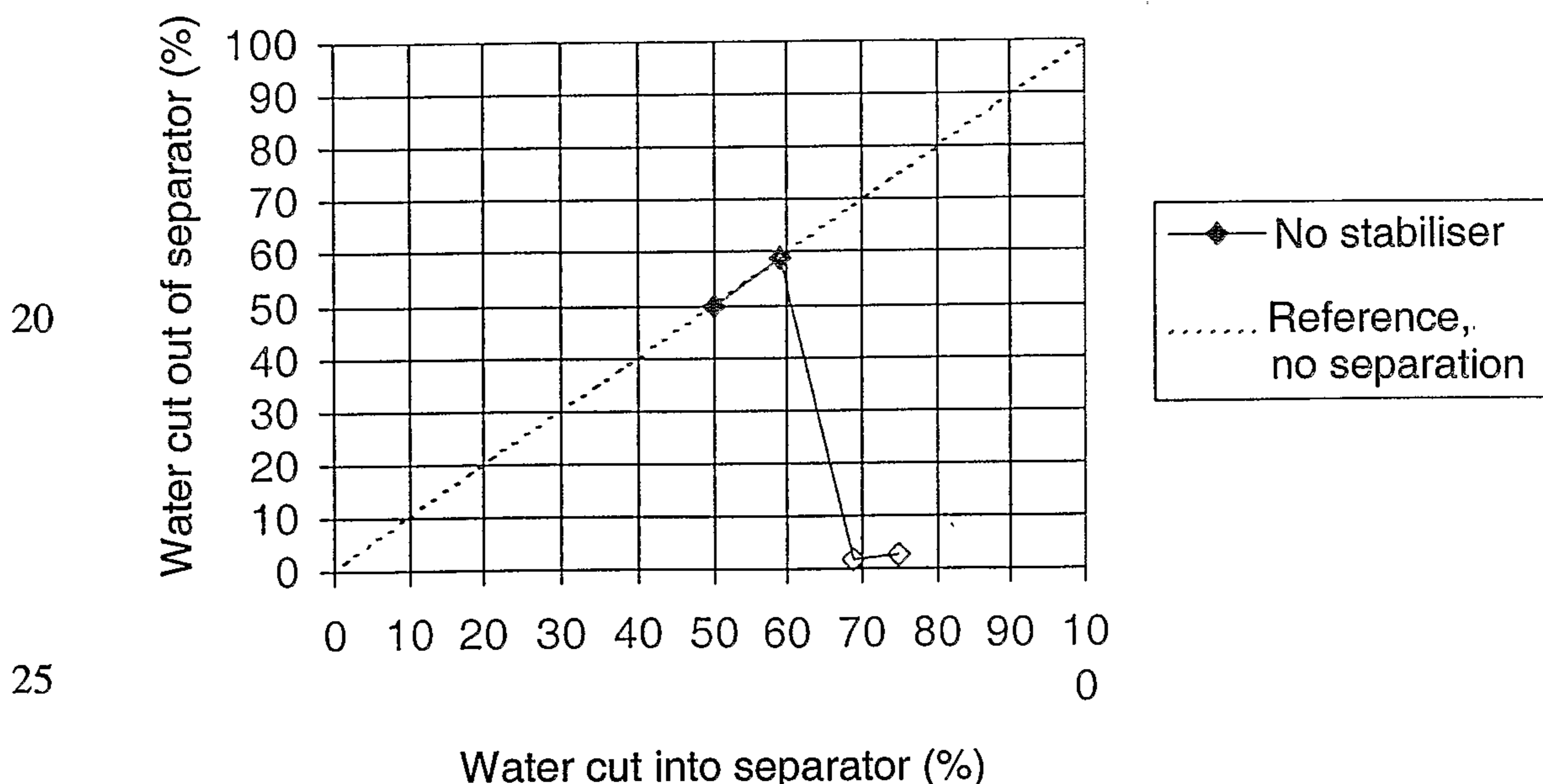
Effect of water recirculation
