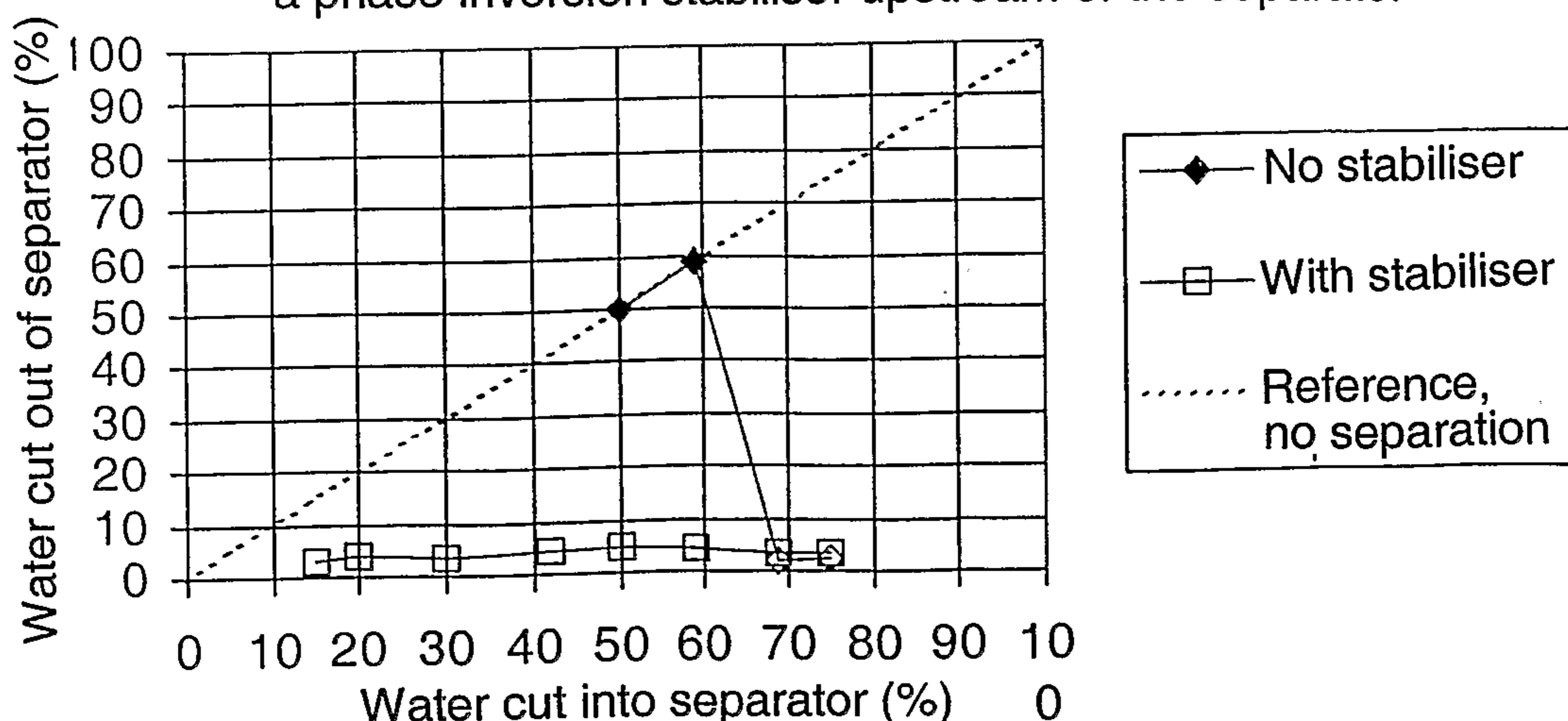
Effect of water recirculation with and without a phase inversion stabiliser upstream of the separator
