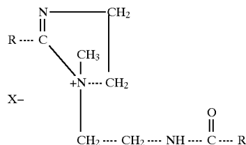
Dialkyl Phenol Alkoxyated Quaternary Ammonium Compound
