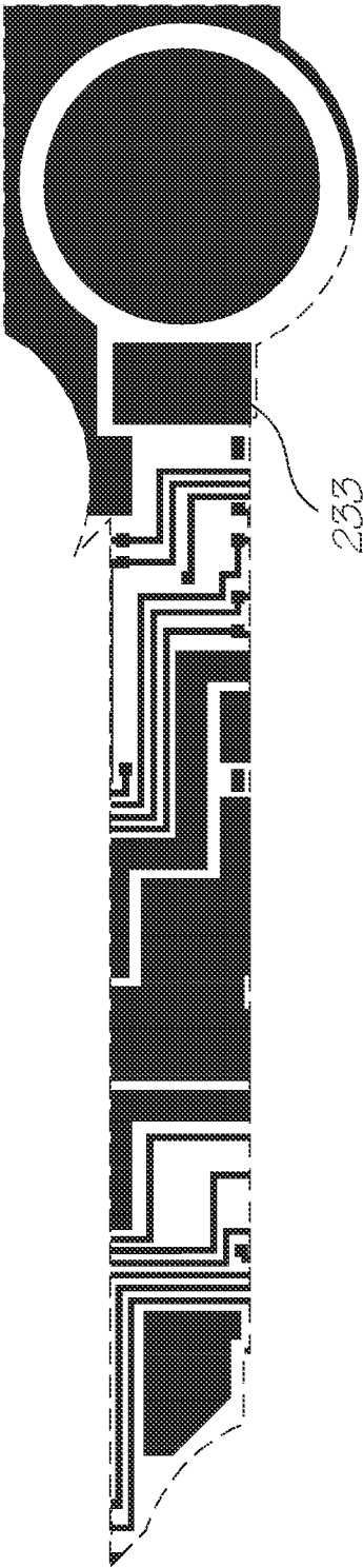
Metal 2 mask
