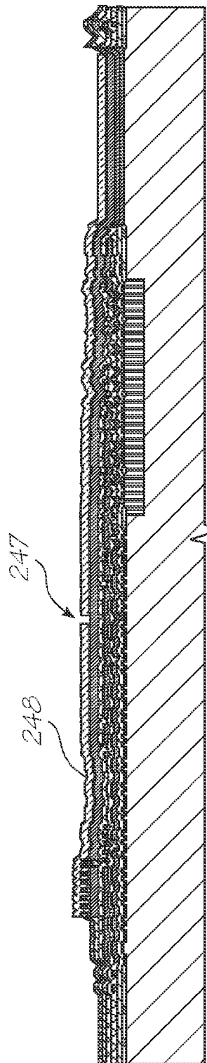
Deposit heater TiN
