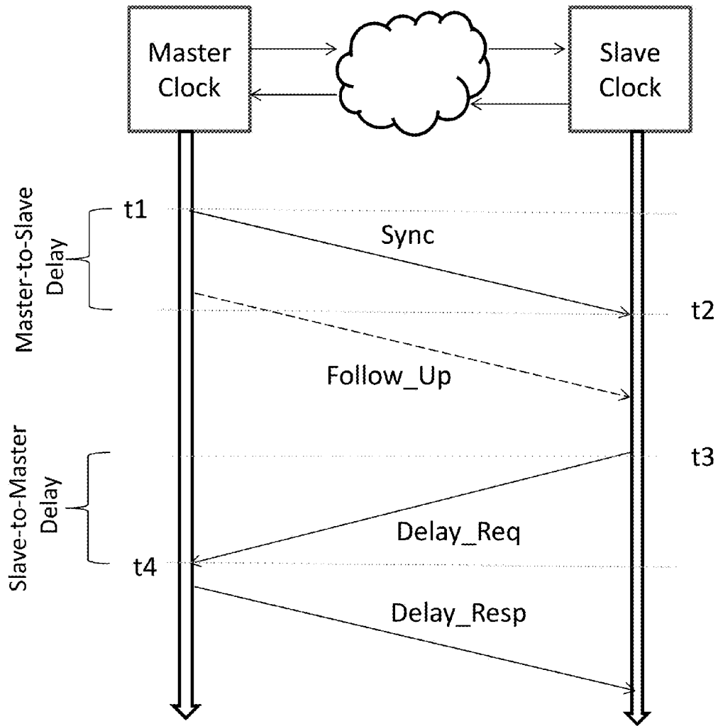
IEEE 1588 Propagation Delay Message Exchange
