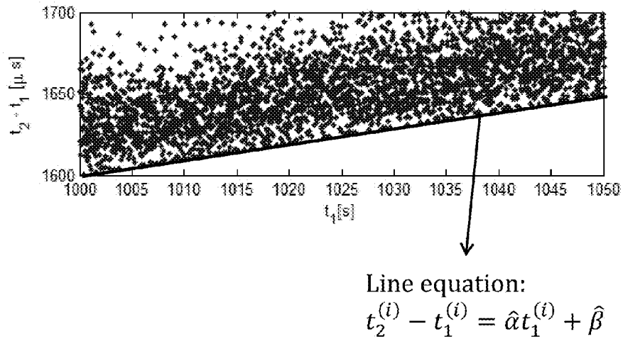
Fig. 4A Before adjusting the frequency
