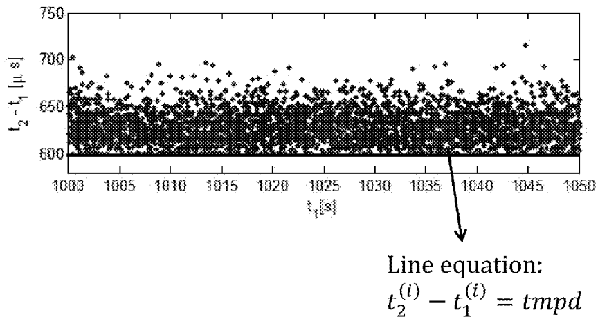
Fig. 4B After adjusting the frequency
