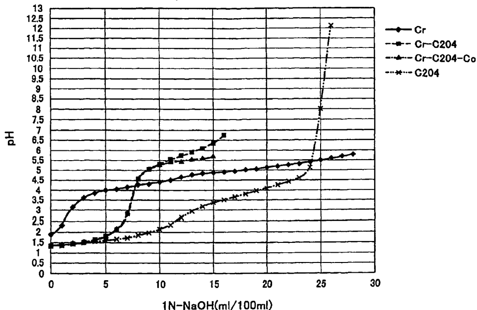
pH curves
