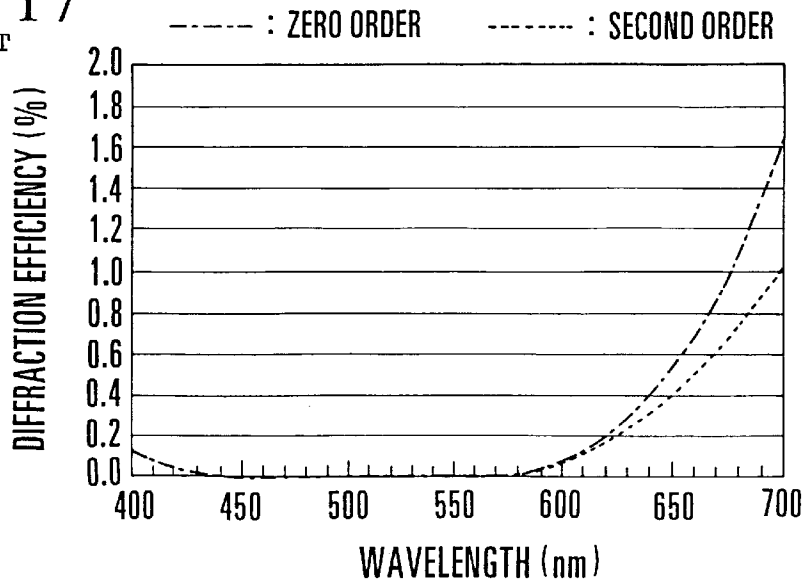
FIG. 18 PRIOR ART
