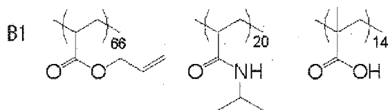
Isomer Mixture
