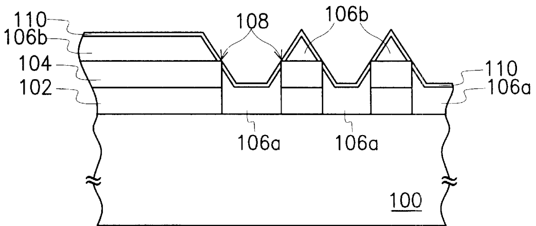
FIG. 1C (PRIOR ART)
