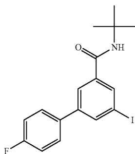
Intermediate 2: N-tert-Butyl-3-(4-fluorophenyl)-5-iodobenzamide
