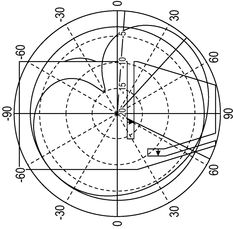
Radiated Power
