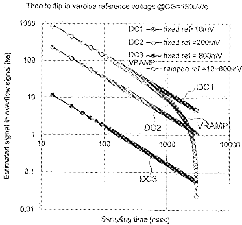
Light to time conversion plot at various reference voltage at comparator input
