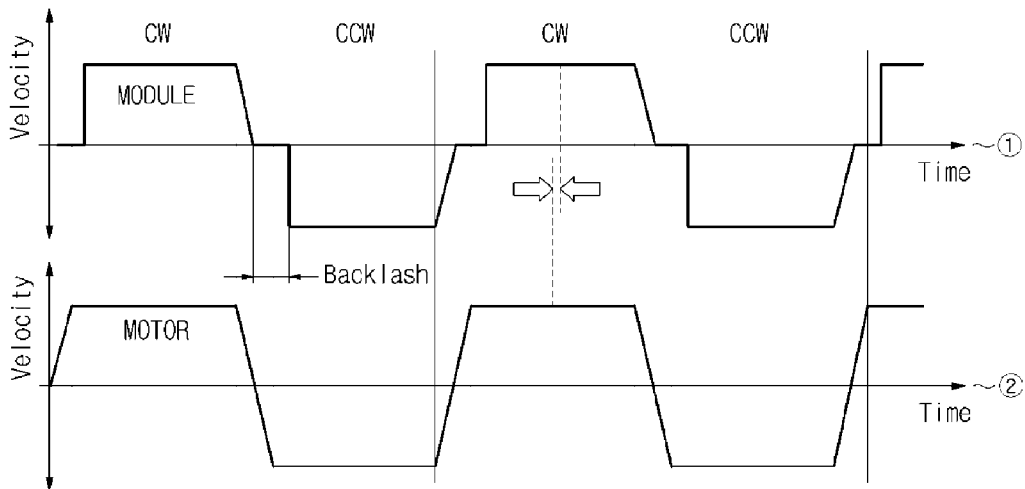
(c) IMAGE BLURRING CAUSED BY BACKLASH
