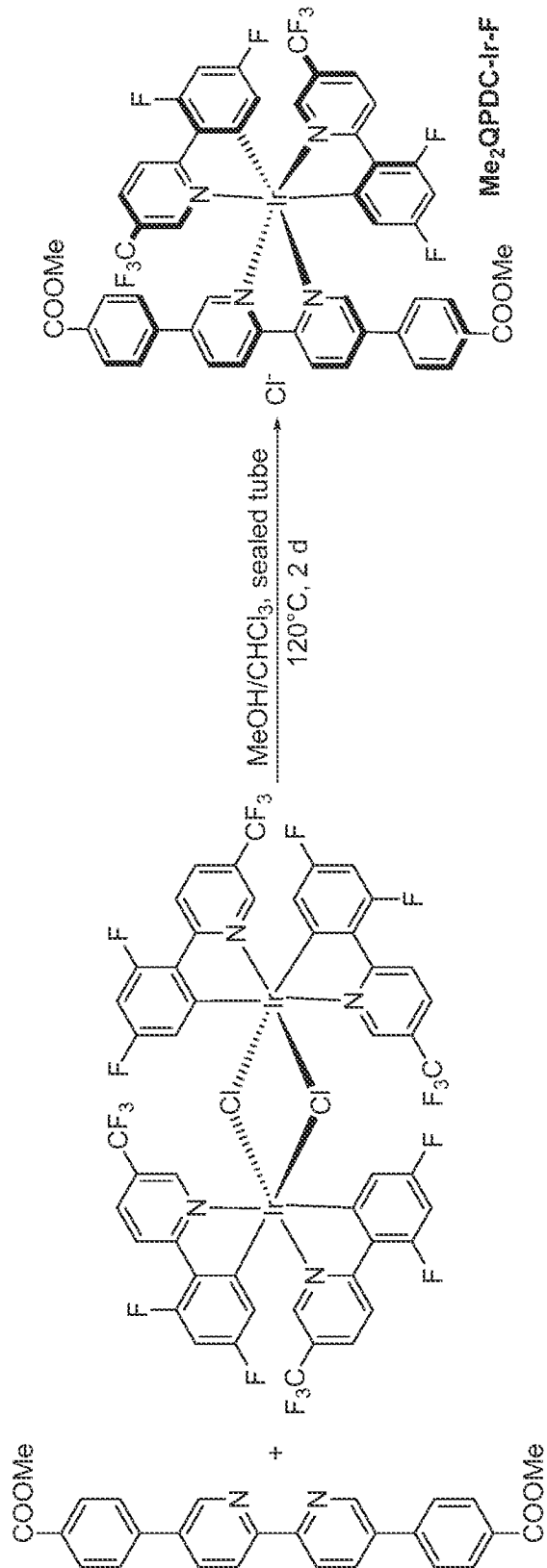
Scheme 10. Synthesis of \text{Me}_2\text{QPDC-Ir-F} ligand.
