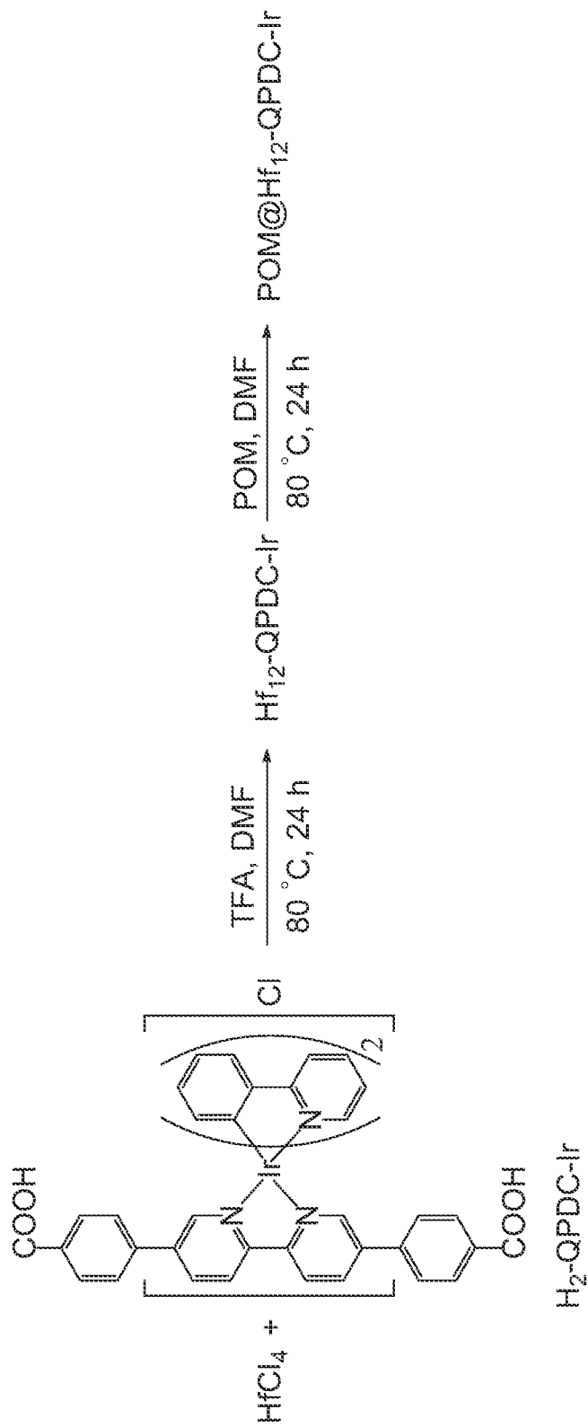
Scheme 9: Synthesis route of POM@Hf 12 -QPDC-Ir.
