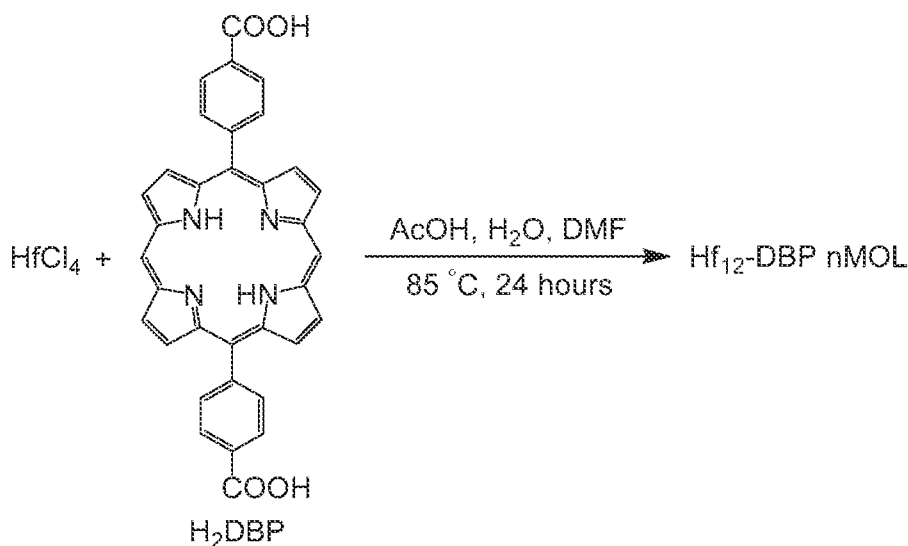
Scheme 14. Synthesis of Hf 12 -DBP nMOL.
