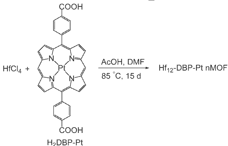
Scheme 8. Synthesis of Hf 12 -DBP-Pt nMOF.
