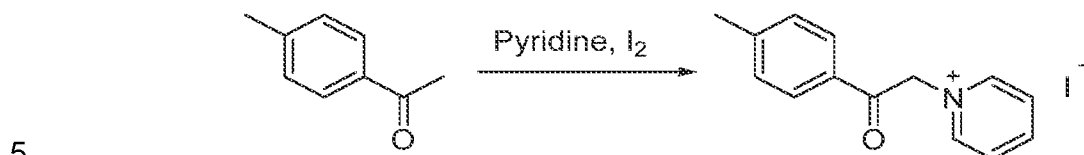
Scheme 2. Synthesis of 1-(2-oxo-2-(p-tolyl)ethyl)pyridin-1-ium.
