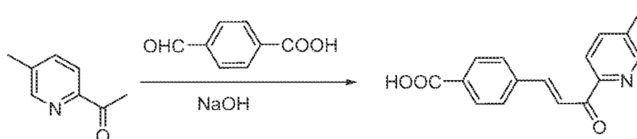
Scheme 1. Synthesis of 4-(5-methylpyridin-2-yl)formylvinyl benzoic acid.
