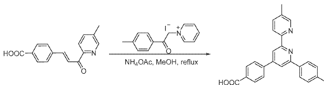
Scheme 3. Synthesis of 4-[2-(4-methylphenyl)-6-(5-methylpyridin-2-yl)pyridin-4-yl]benzoic acid.
