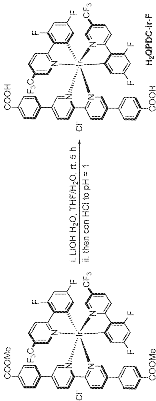
Scheme 11. Synthesis of H 2 QPDC-Ir-F ligand.
