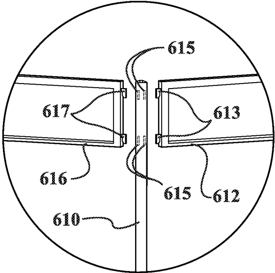
Detail "I" FIG. 45
