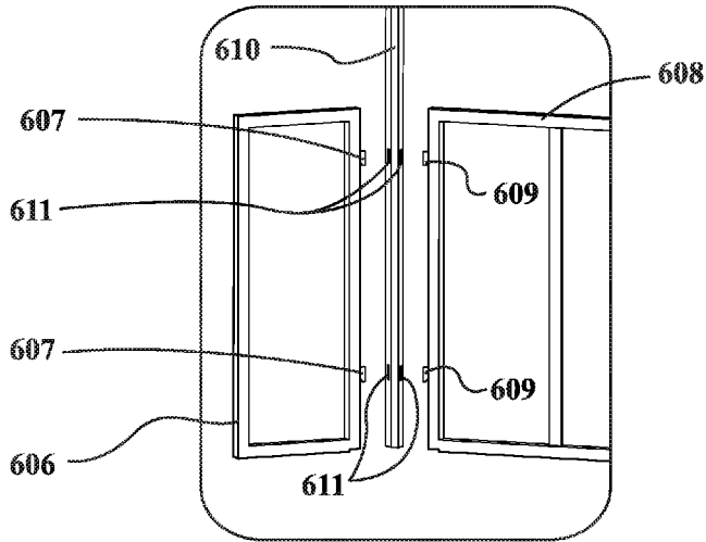
Detail "G" FIG. 43
