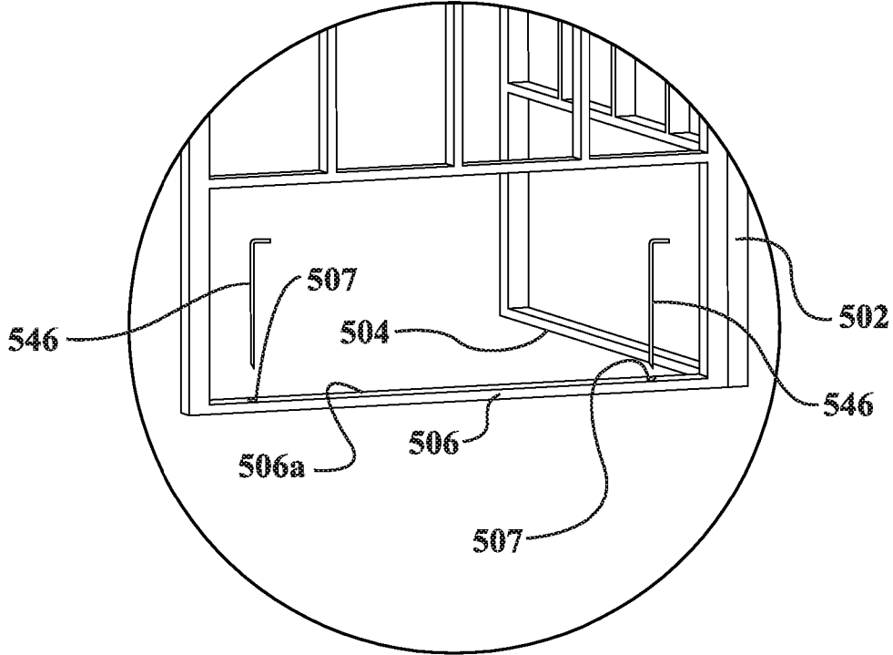
Detail "F" FIG. 36
