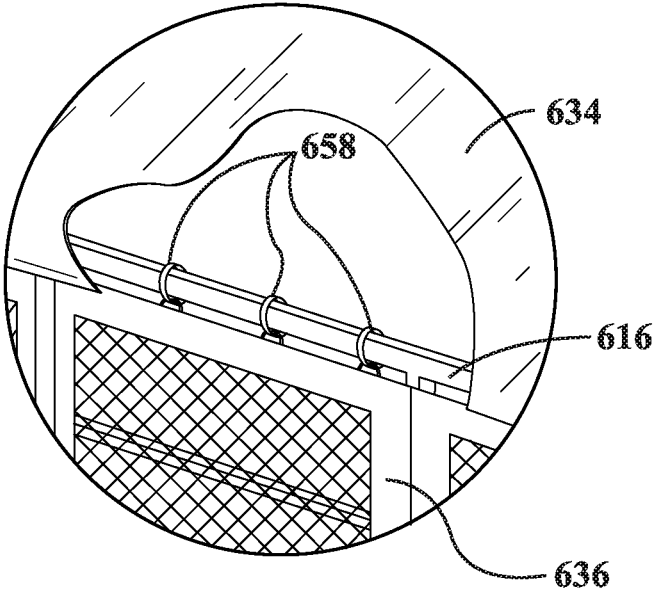
Detail "J" FIG. 46
