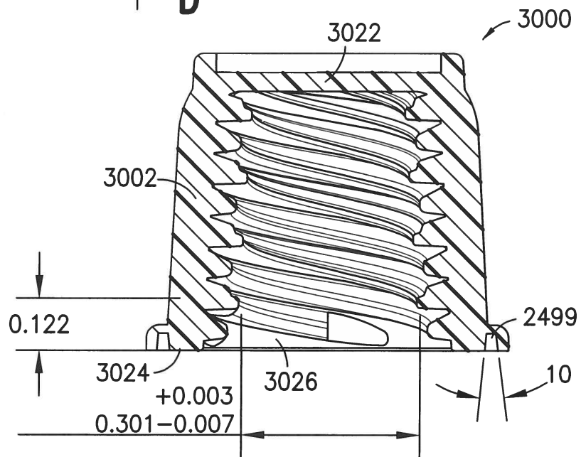
SECTION AC-AC
