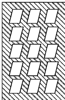
PARALLELOGRAM- SHAPED MOLD TRAY (TOP VIEW) FIG. 35
