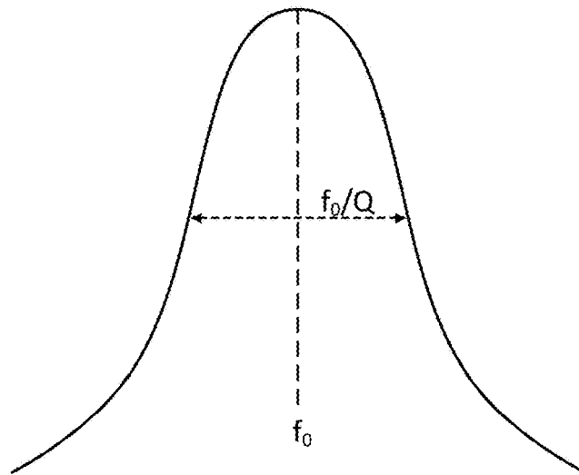
FIG. 4 PRIOR ART
