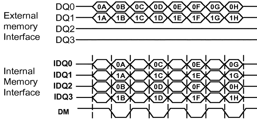
Timing Chart 3000
