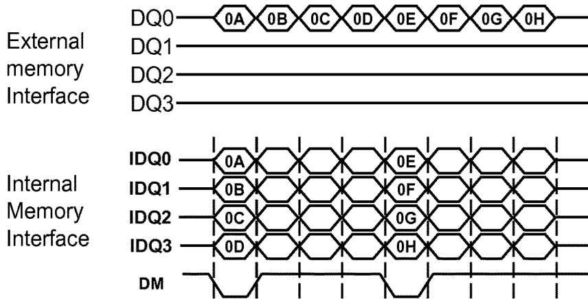
Timing Chart 3001
