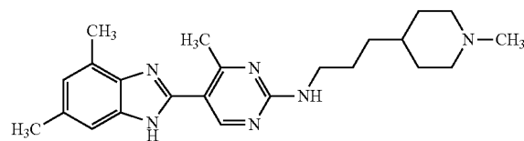
[5-(4,6-Dimethyl-1H-benzoimidazol-2-yl)-4-methyl-pyrimidin-2-yl]-[3-(1-methyl-piperidin-4-yl)-propyl]-amine
