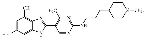
[5-(4,6-Dimethyl-1H-benzoimidazol-2-yl)-4-methyl-pyrimidin-2-yl]-[3-(1-methyl-piperidin-4-yl)-propyl]-amine
