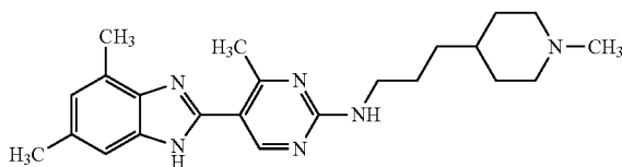
[5-(4,6-Dimethyl-1H-benzoimidazol-2-yl)-4-methyl-pyrimidin-2-yl]-[3-(1-methyl-piperidin-4-yl)-propyl]-amine
