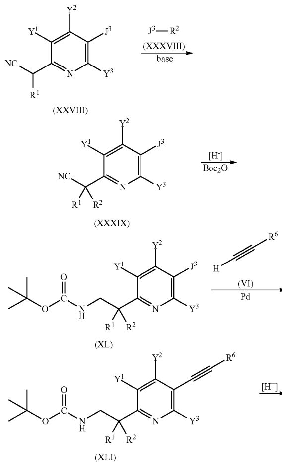
Reaction Scheme 6
