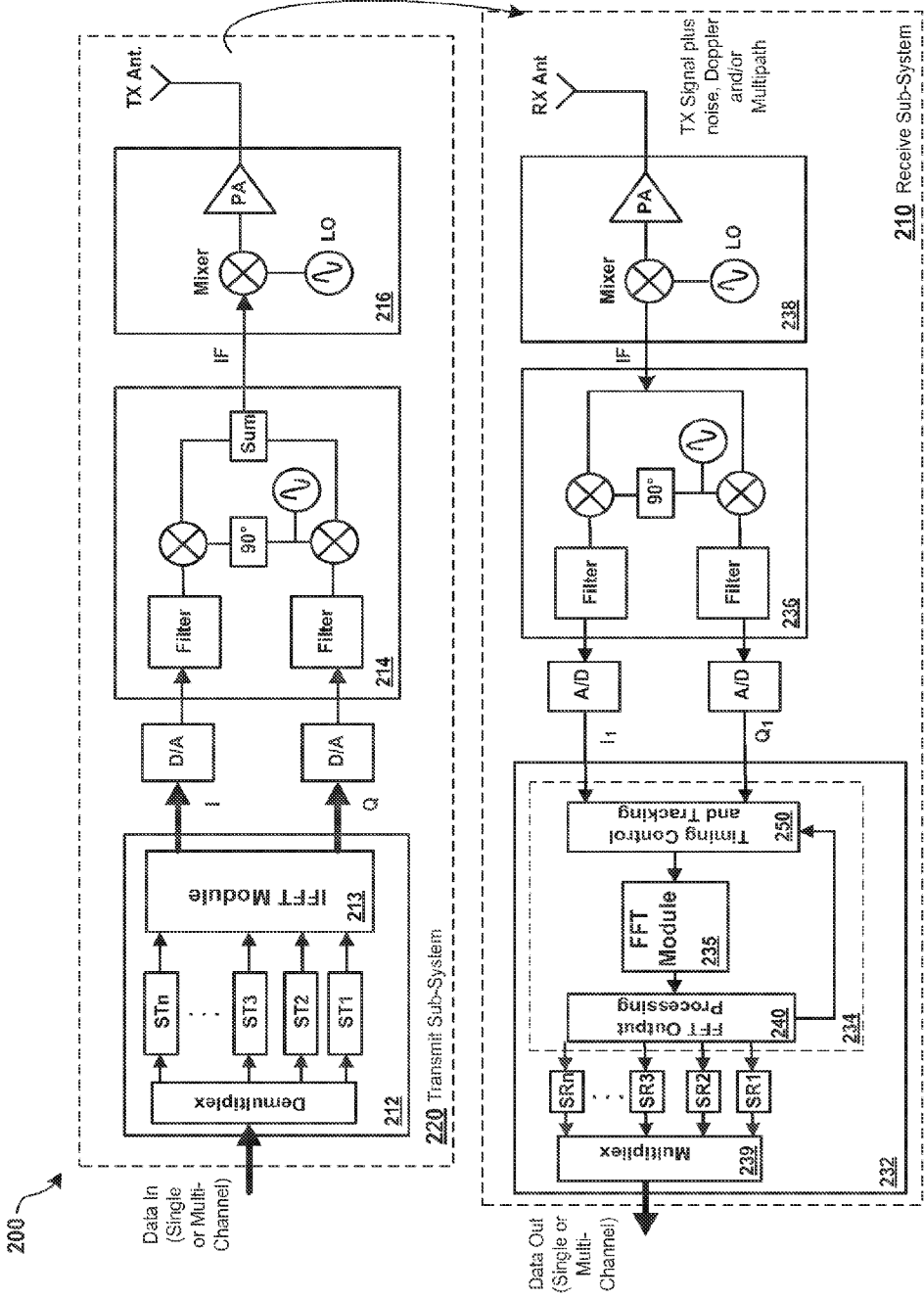
FIG. 2 OFDM Communications System Transmit and Receive Sub-Systems
