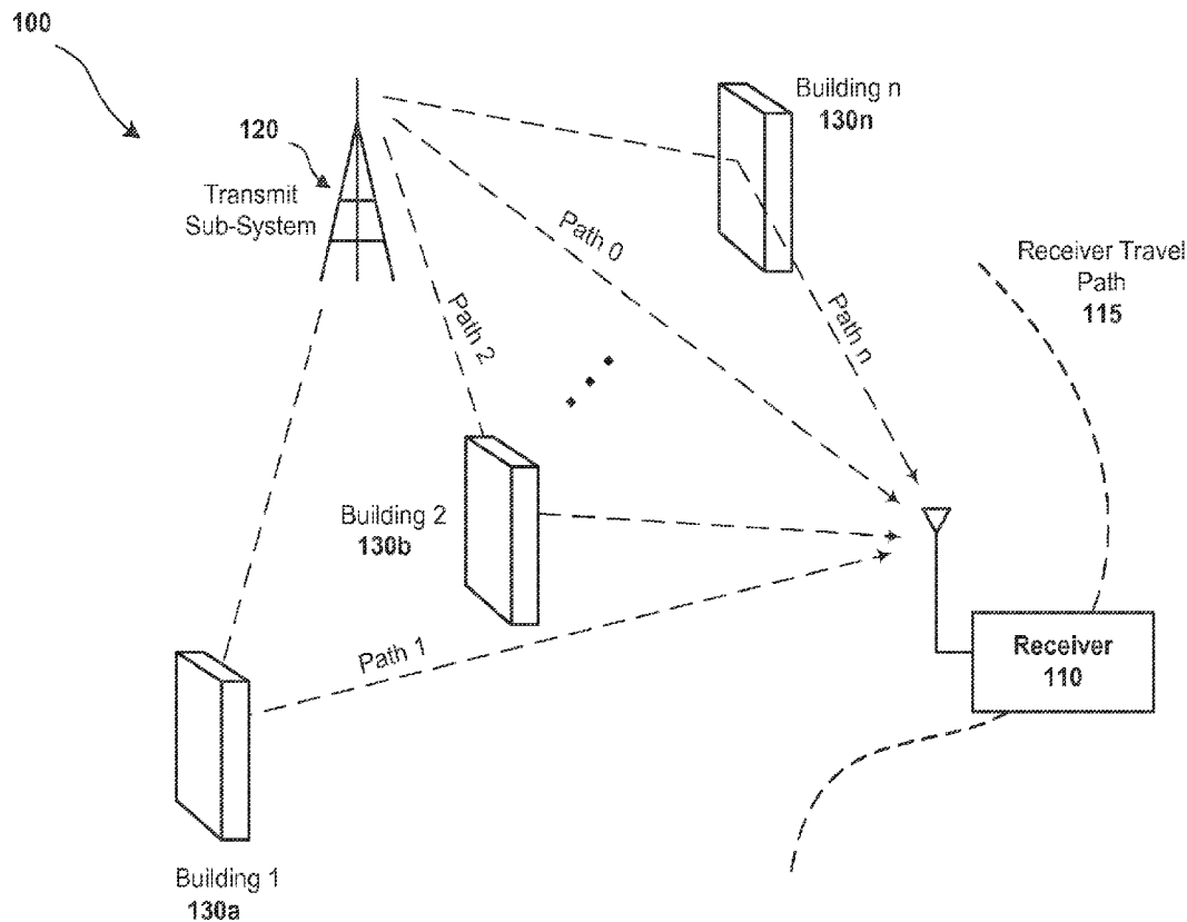
Typical Communications System Affected by Multipath Interference
