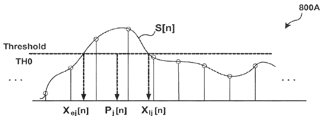
FIG. 8A Example of Peak Determination
