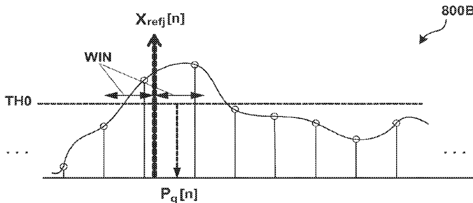
FIG. 8B Example of Peak Tracking and Updating
