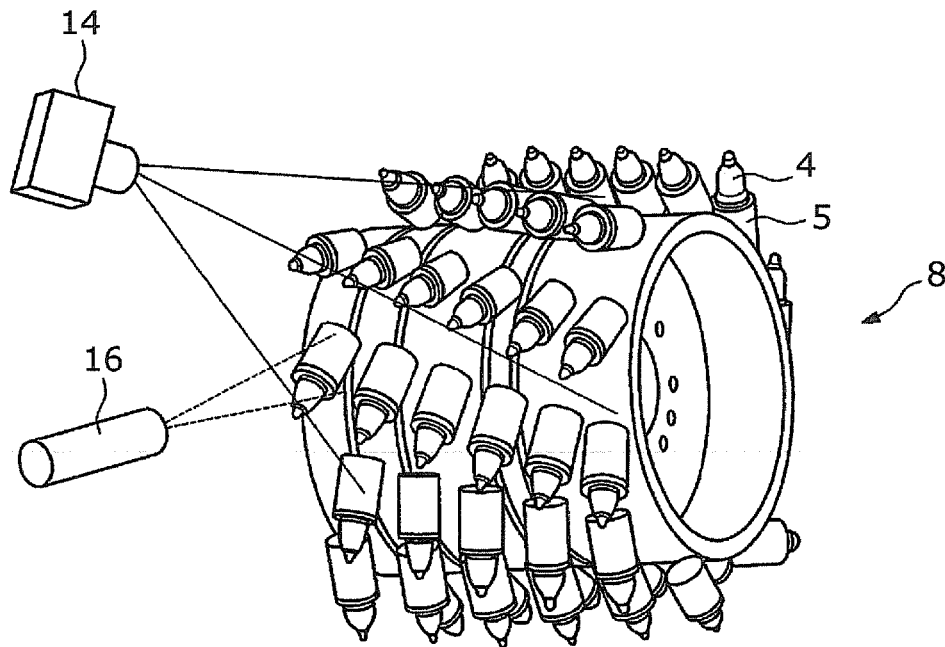
Fig. 3 (prior art)
