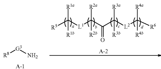
GENERAL REACTION SCHEME 1
